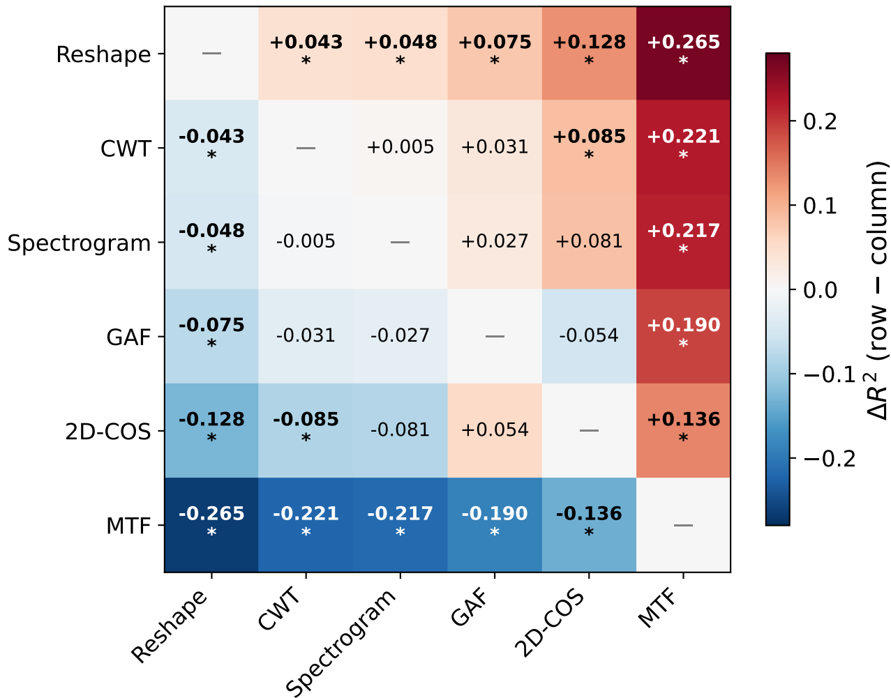
Pairwise \Delta R^2 between transforms (* = significant after Bonferroni correction, \alpha = 0.003 )
