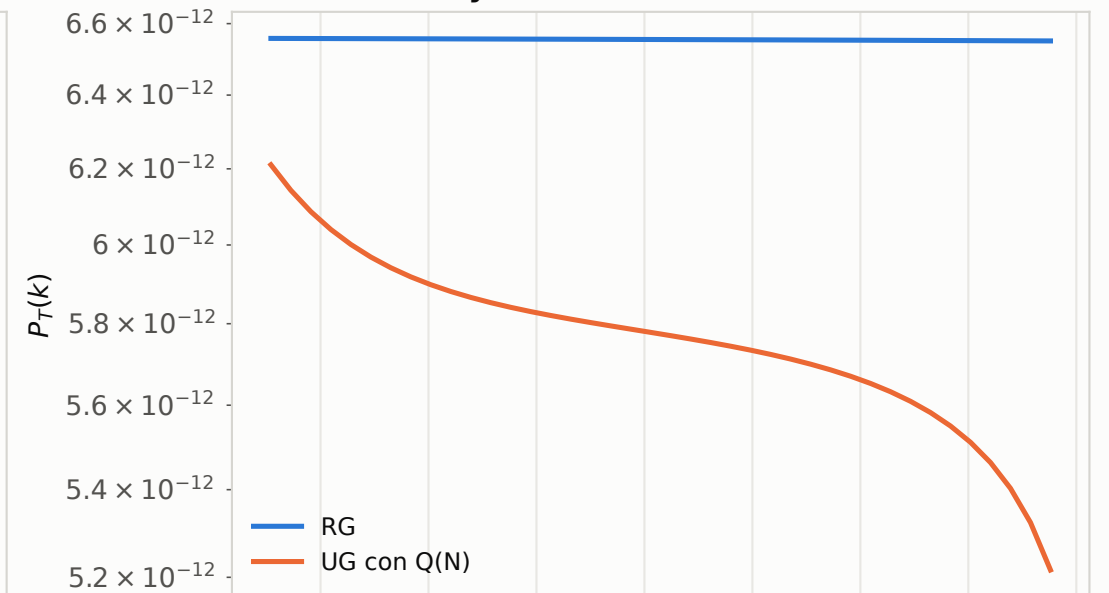
(b) Starobinsky
