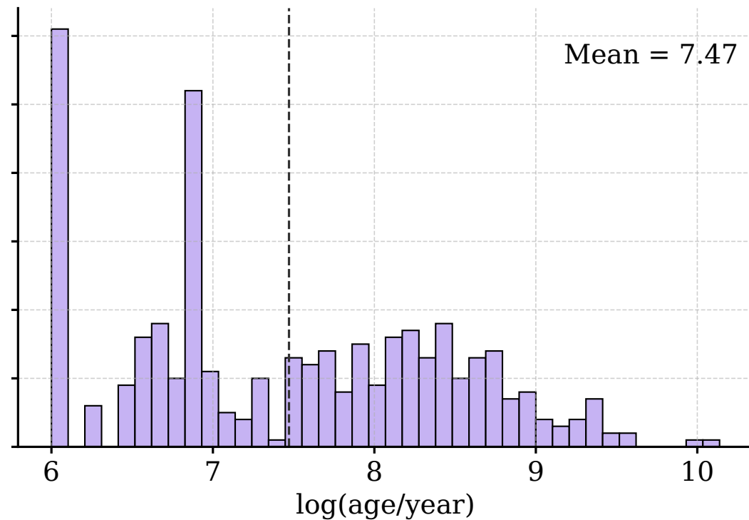
Ts. Clusters of Far Galaxies (n=414)
