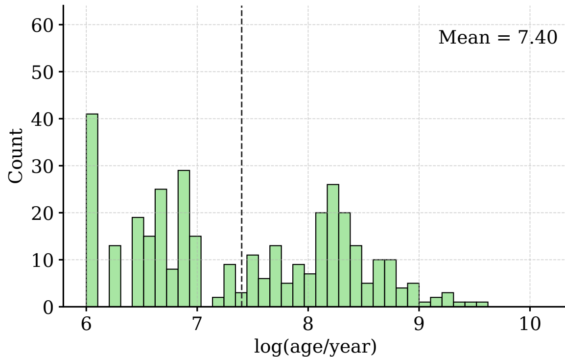
Ts. Clusters of Near Galaxies (n=352)
