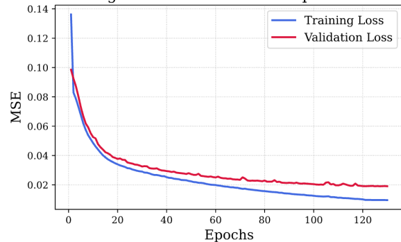
Training and Validation Mean Squared Errors
