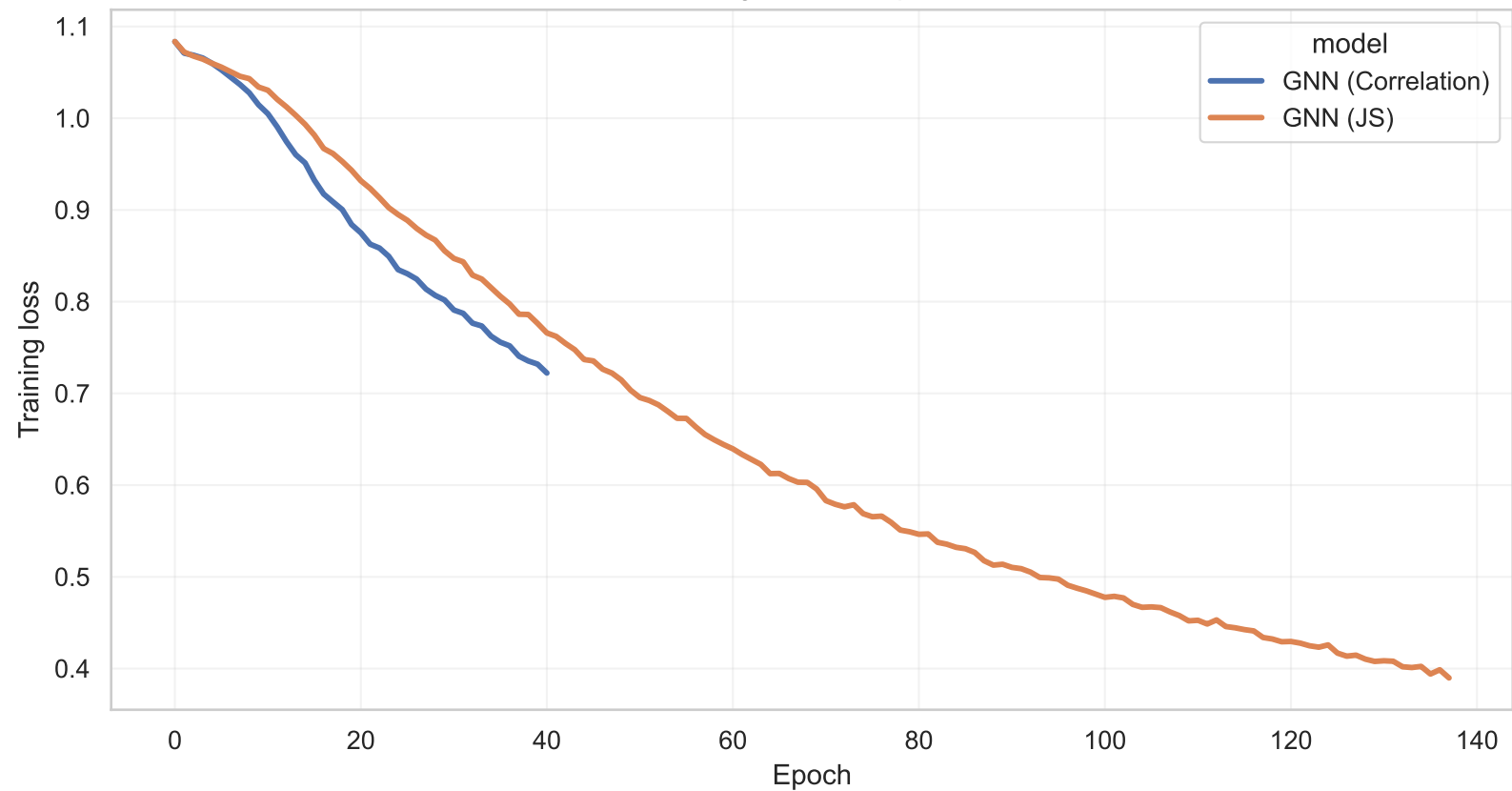
Training loss over epochs
