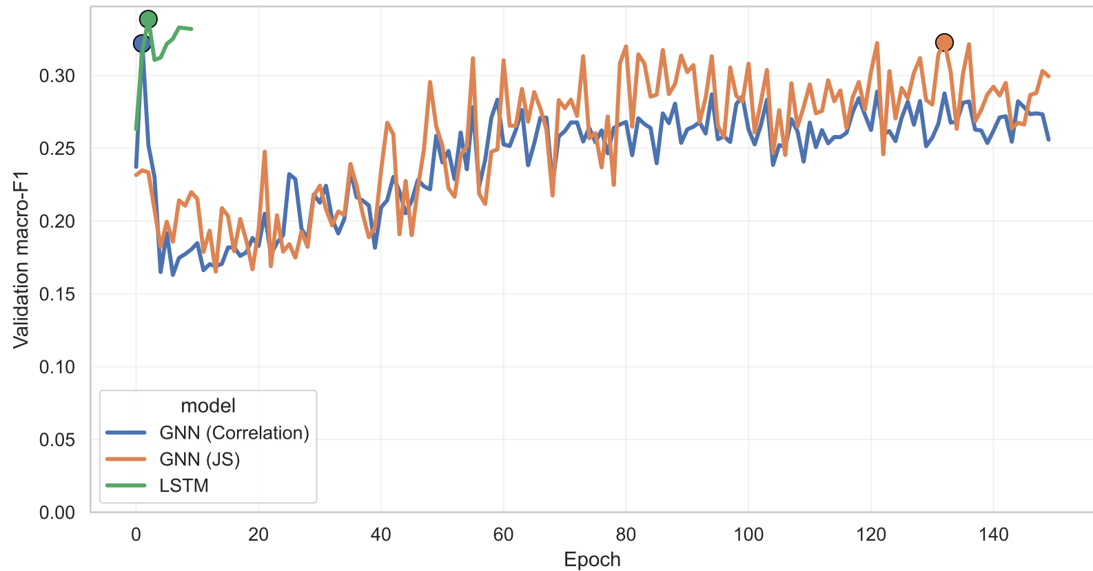
Validation macro-F1 over training
