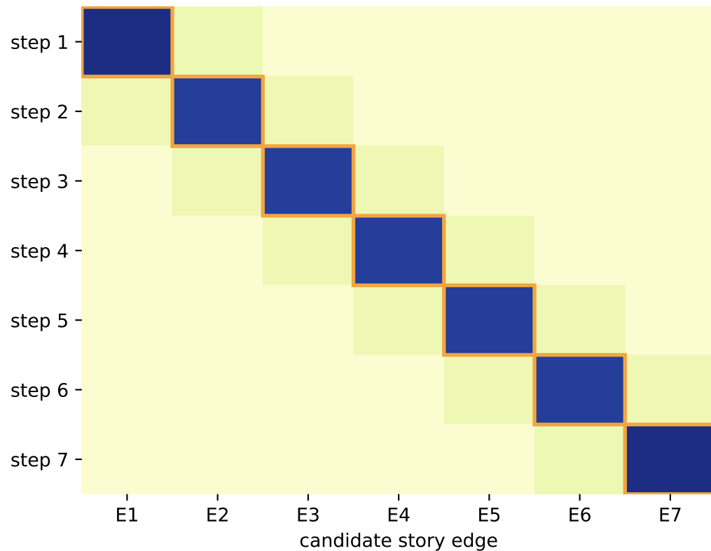
TSRA reasoning attention (trace-aligned next-step selection)
