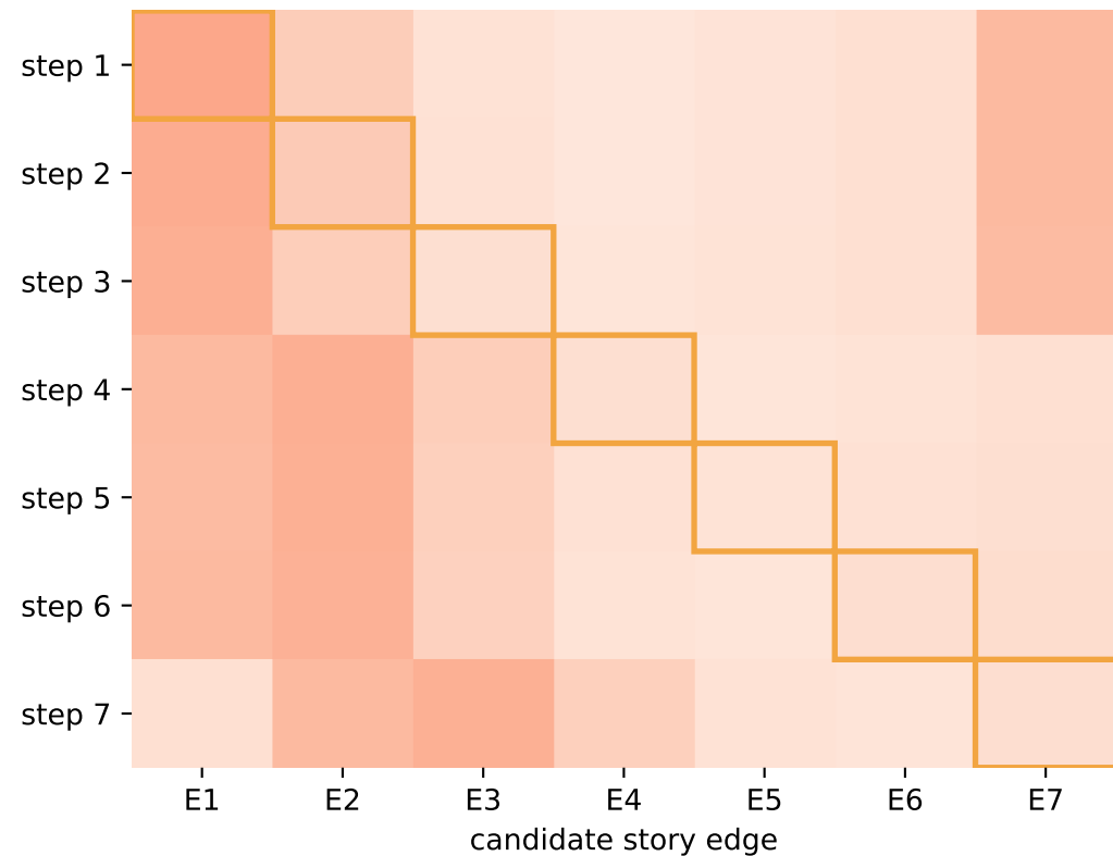
Label-only / vanilla signal (diffuse shortcut attention)
