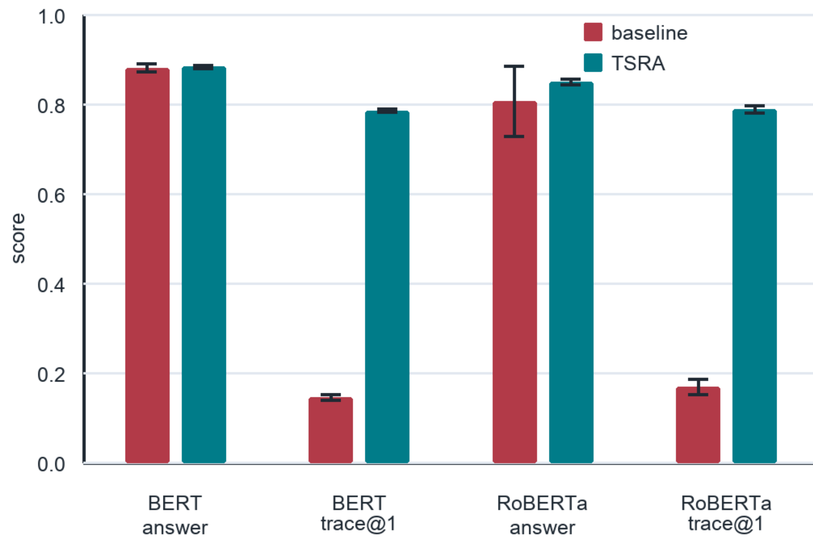
ProofWriter depth-5: answer vs trace alignment
