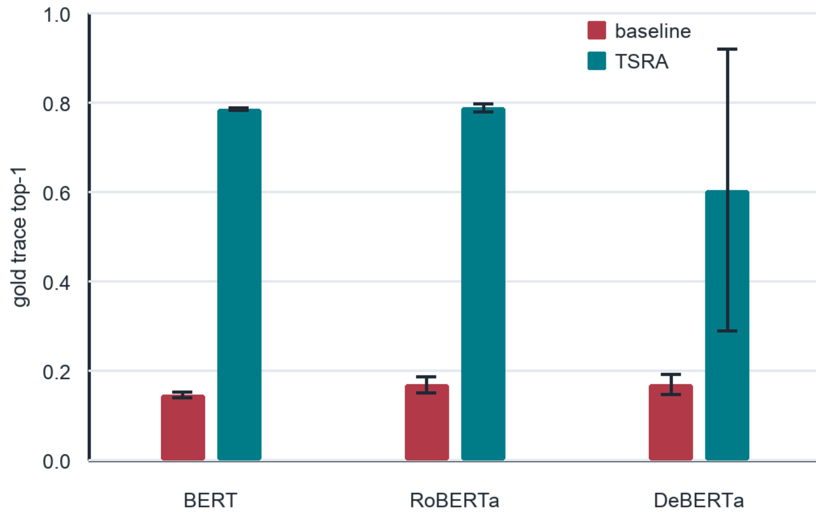
ProofWriter depth-5: trace@1
