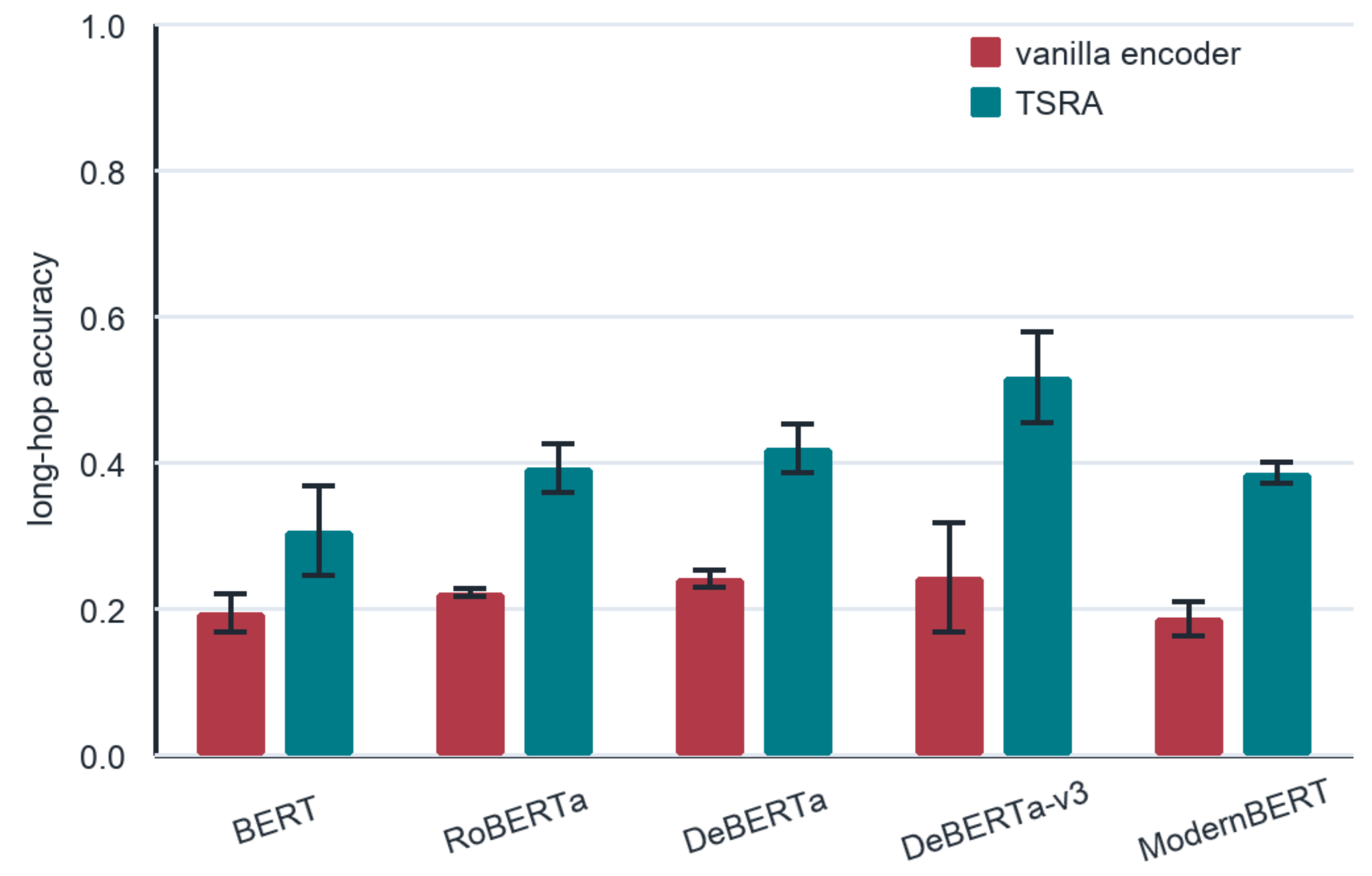
CLUTRR 2/3-hop train -> 6-10-hop test
