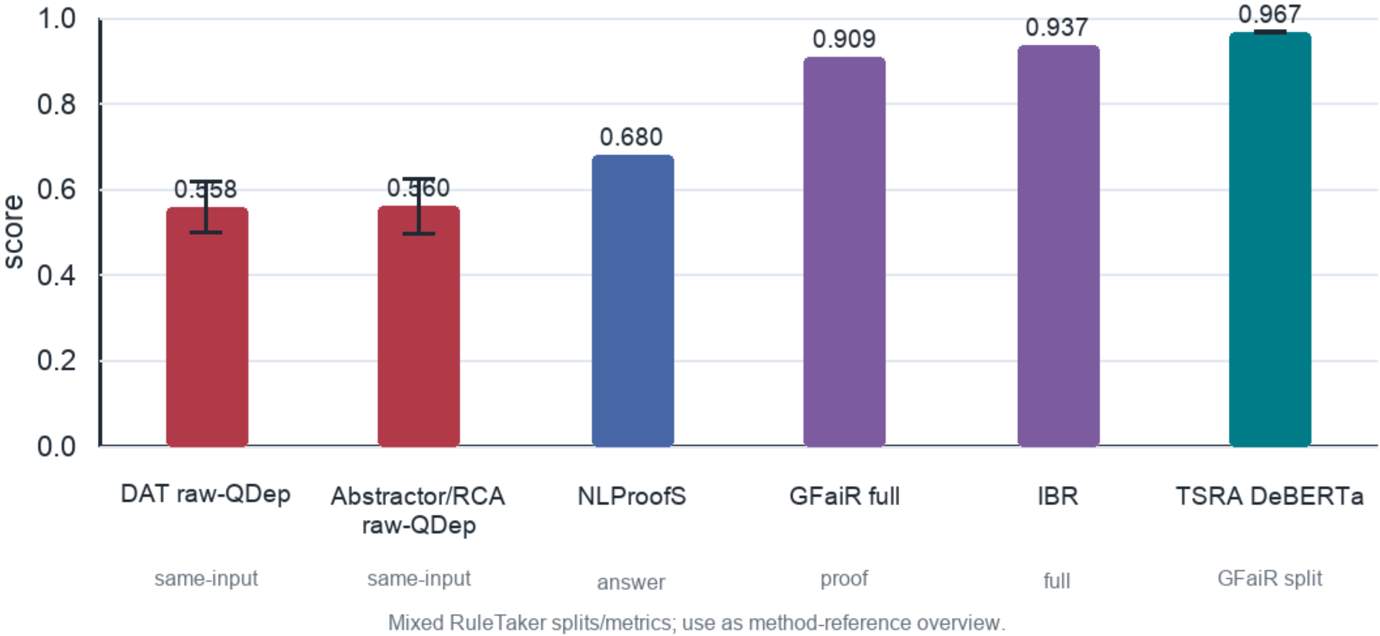
RuleTaker result comparison
