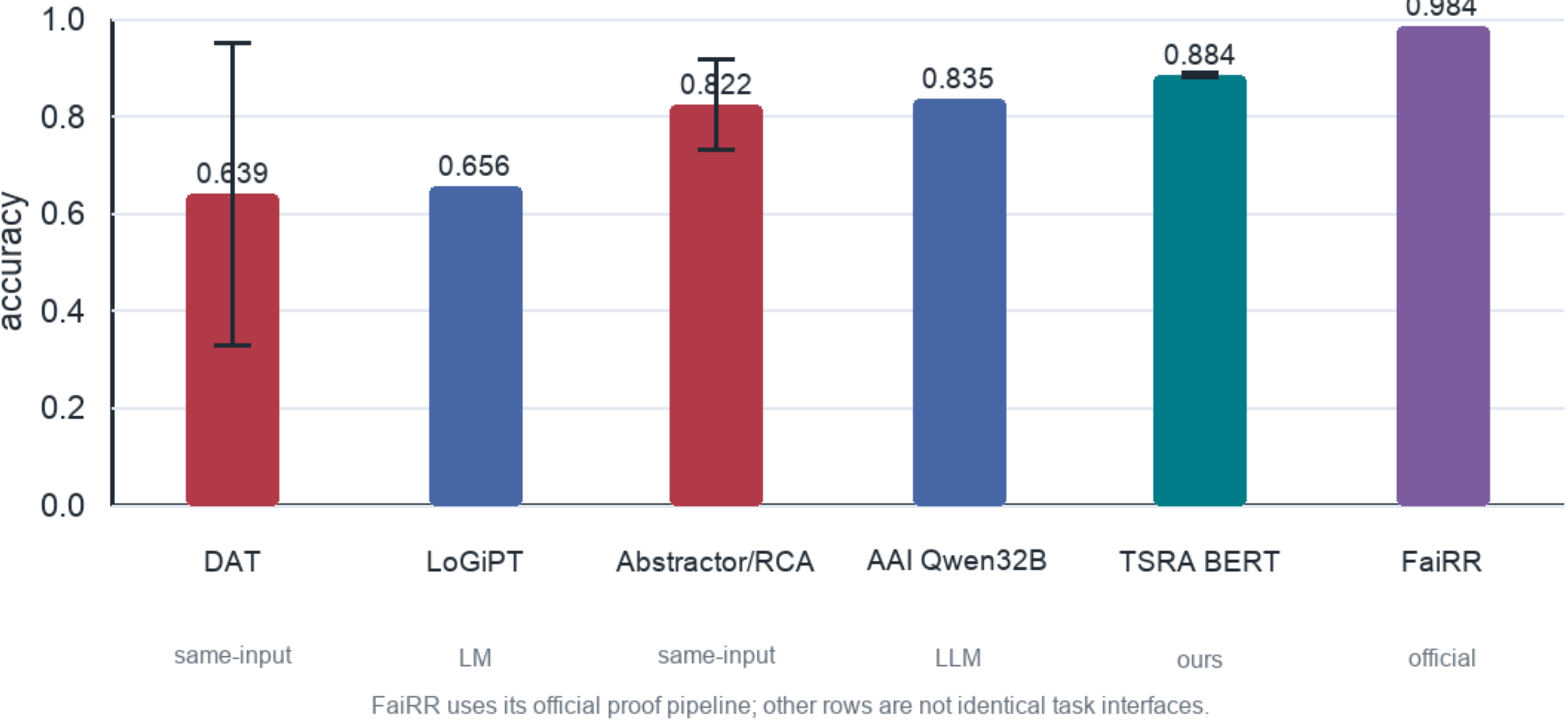
ProofWriter depth-5 accuracy
