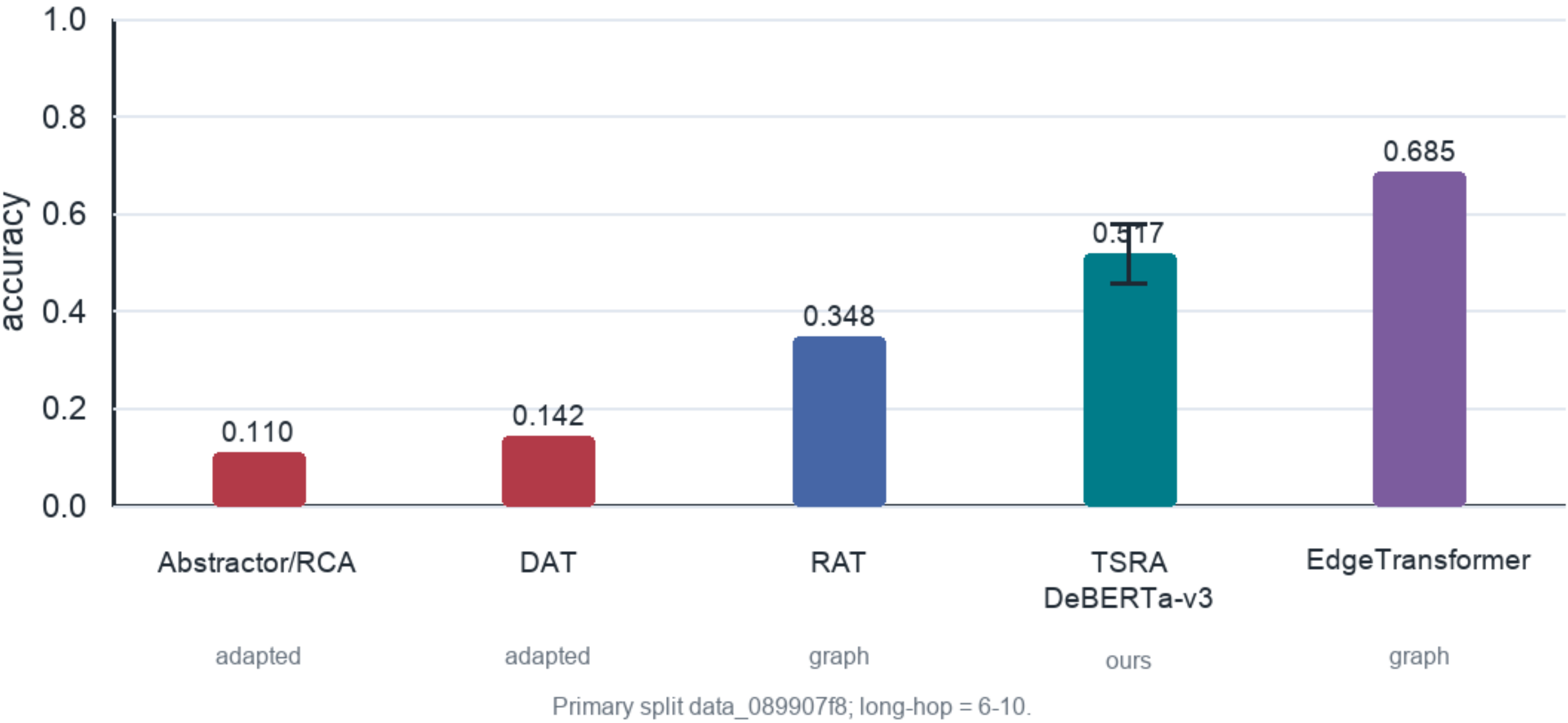
CLUTRR long-hop accuracy
