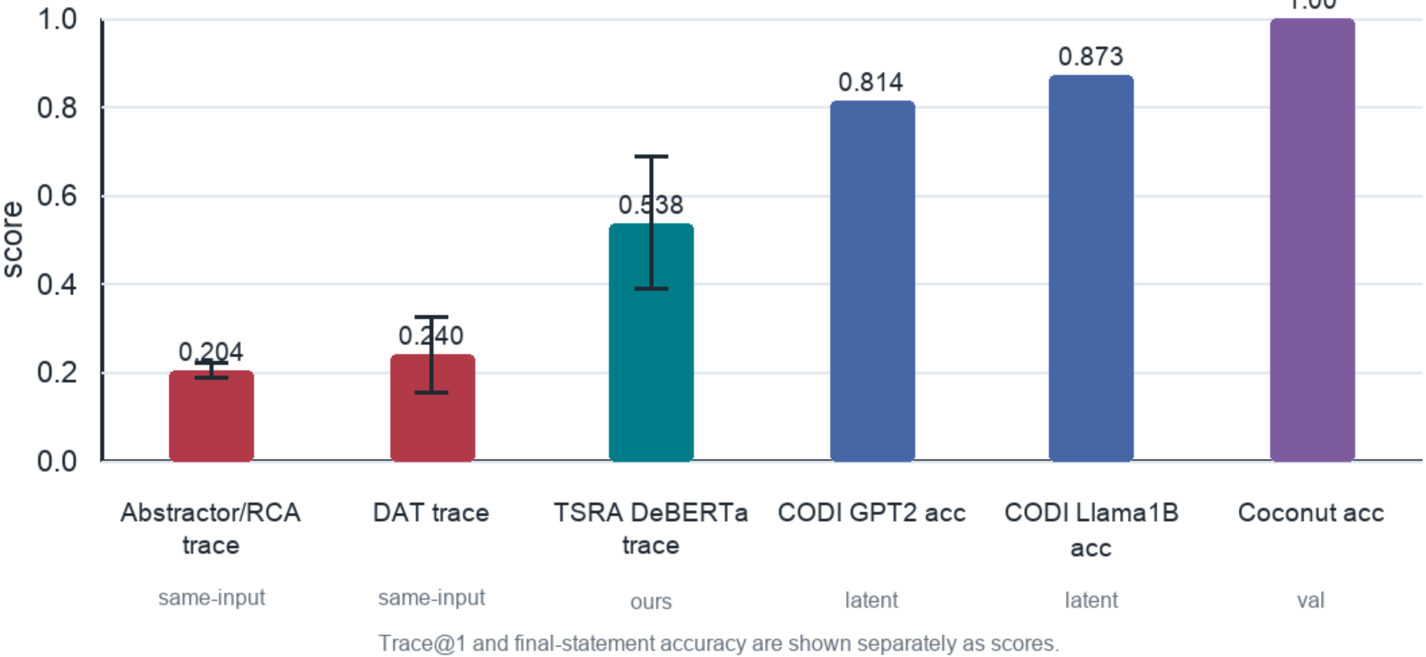
PrOntoQA-OOD trace / latent references
