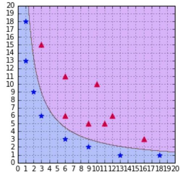
A SVM using a polynomial kernel is able to separate the data (degree=2)
