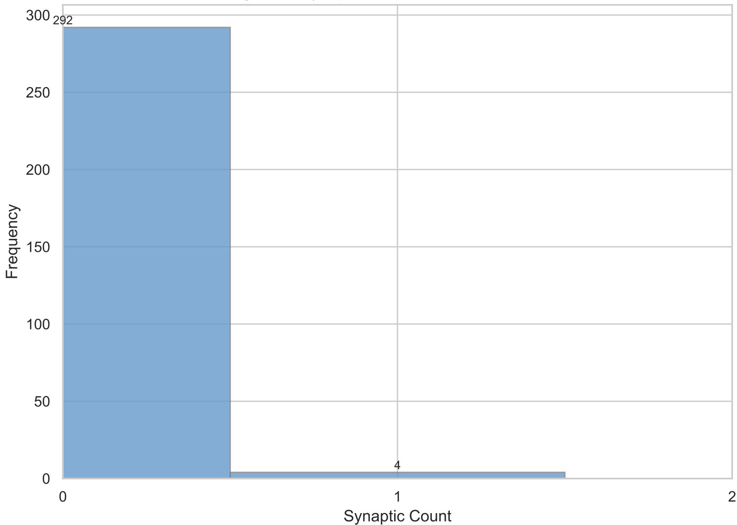
Histogram of Synaptic Counts for Shared Connections
