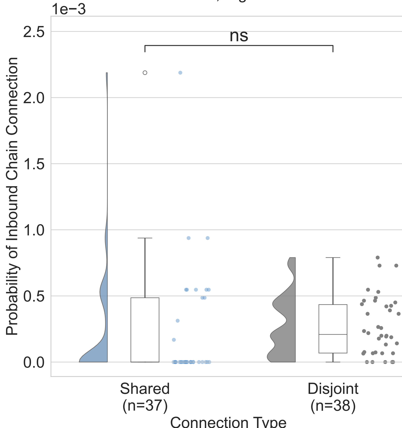
Probability of Inbound Chain Connection by Cell Rank-Sum P-value: 0.99, Signed-Rank P-value: 0.89
