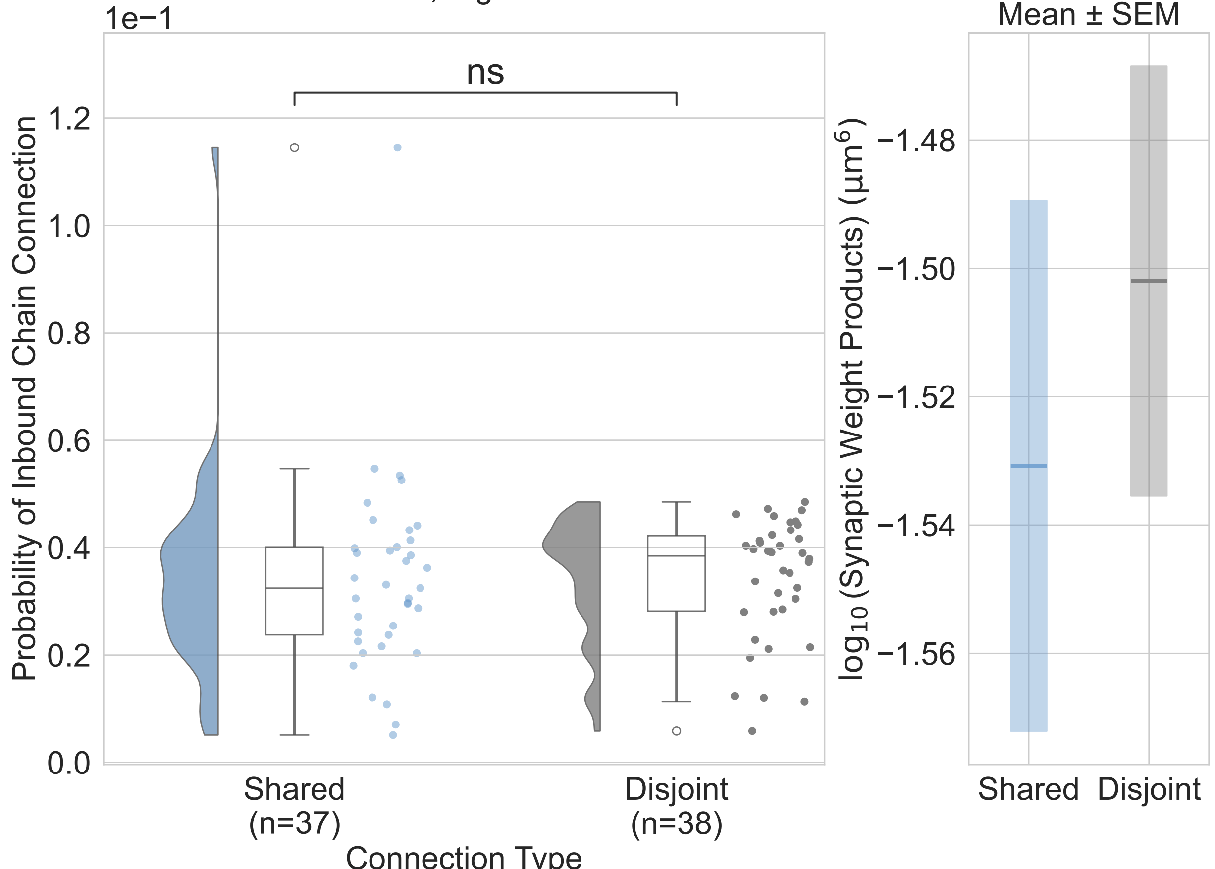
Probability of Inbound Chain Connection by Cell Rank-Sum P-value: 0.17, Signed-Rank P-value: 0.061
