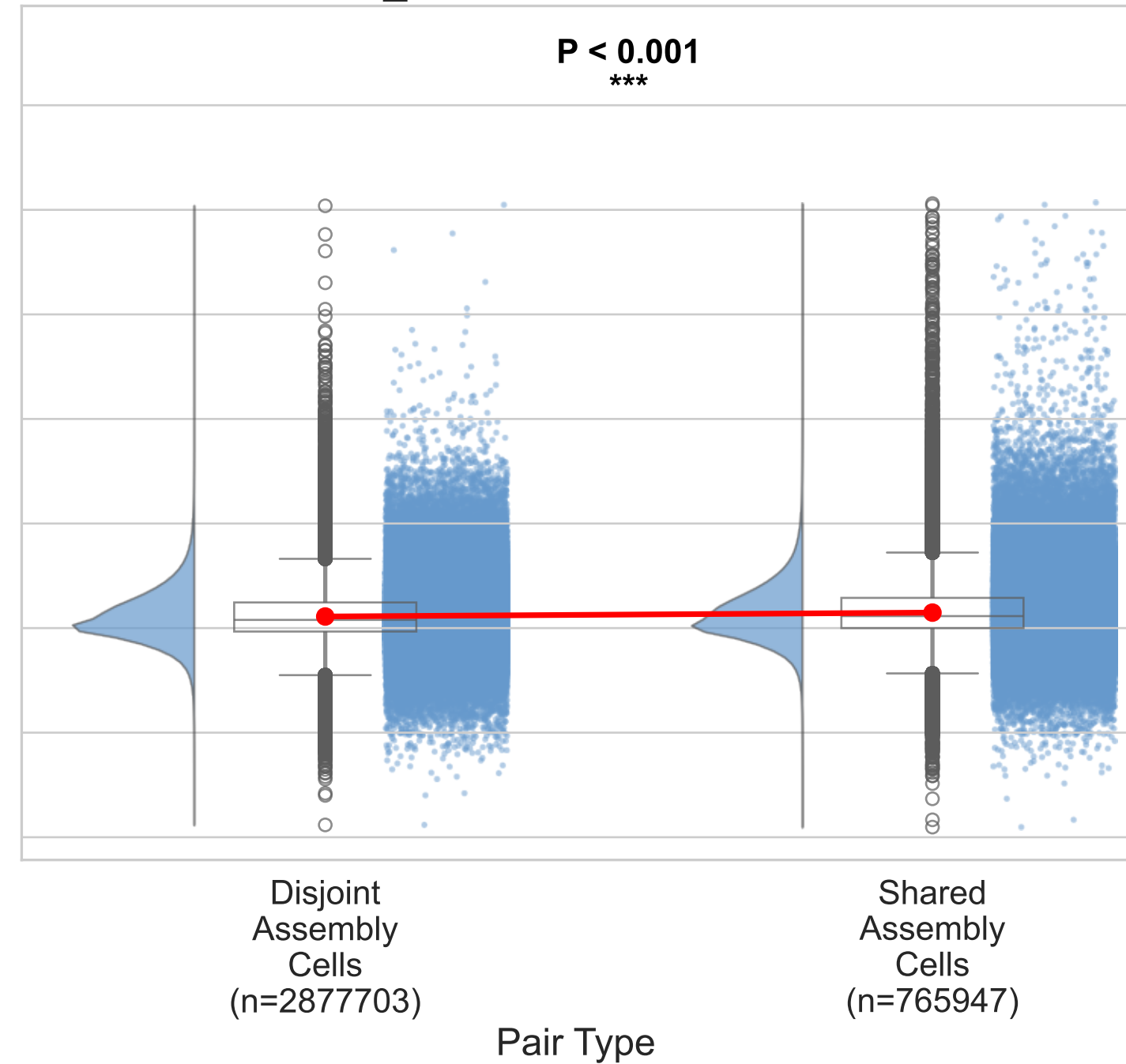
natural_movie – noise correlations
