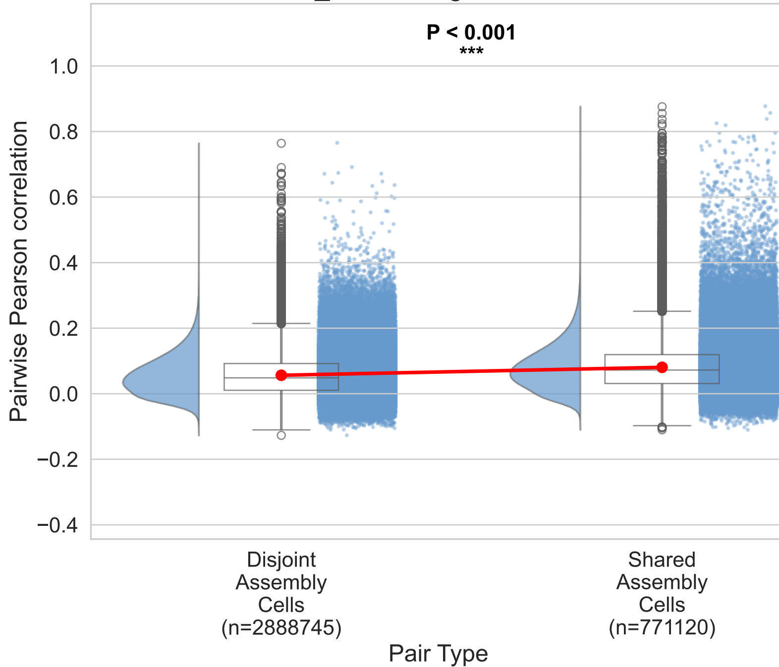
natural_movie – signal correlations
