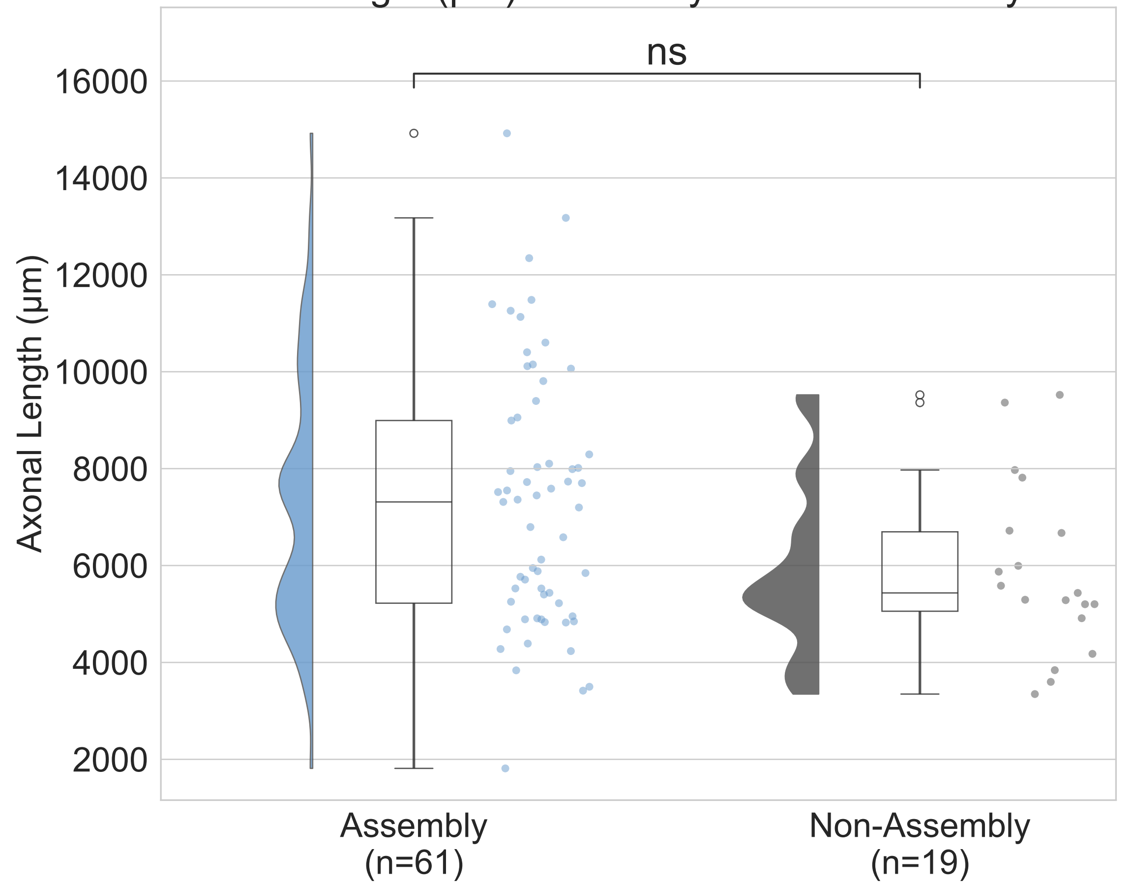
Total Axonal Length ( \mu\text{m} ): Assembly vs Non-Assembly Pre C
