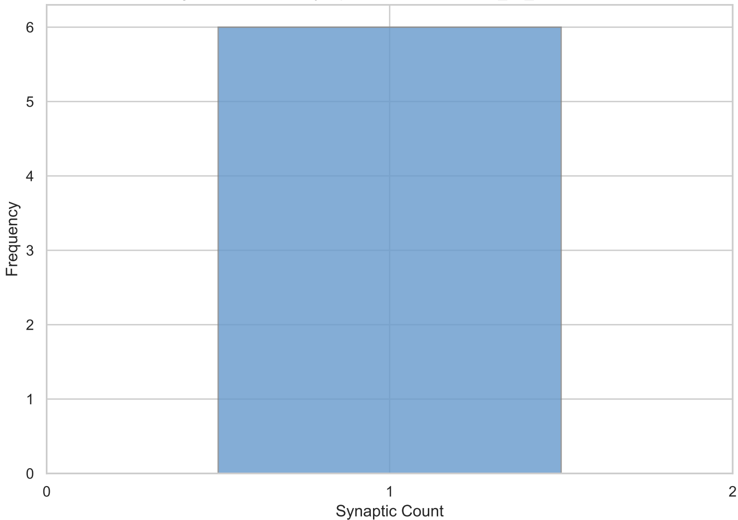
Histogram of Nonzero Synaptic Counts for Shared_no_a Connections 6
