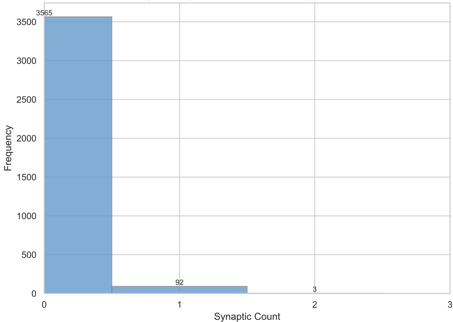
Histogram of Synaptic Counts for Shared_a Connections
