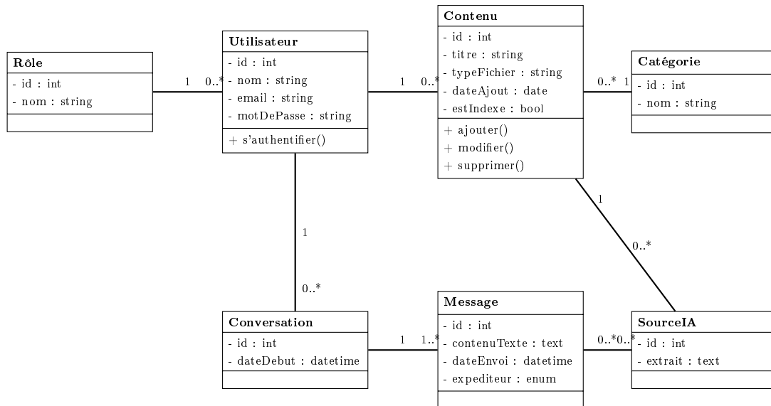
Figure 2.5: Diagramme de classes
