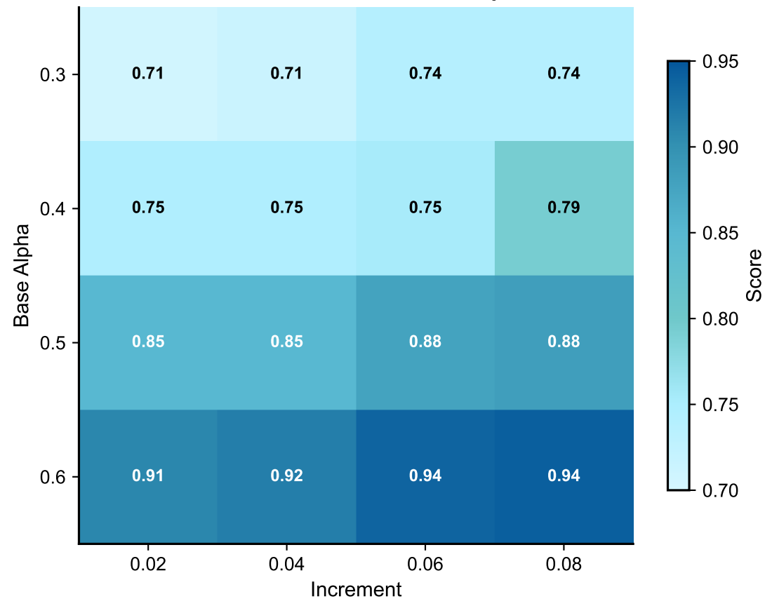
Grid Search Score Heatmap
