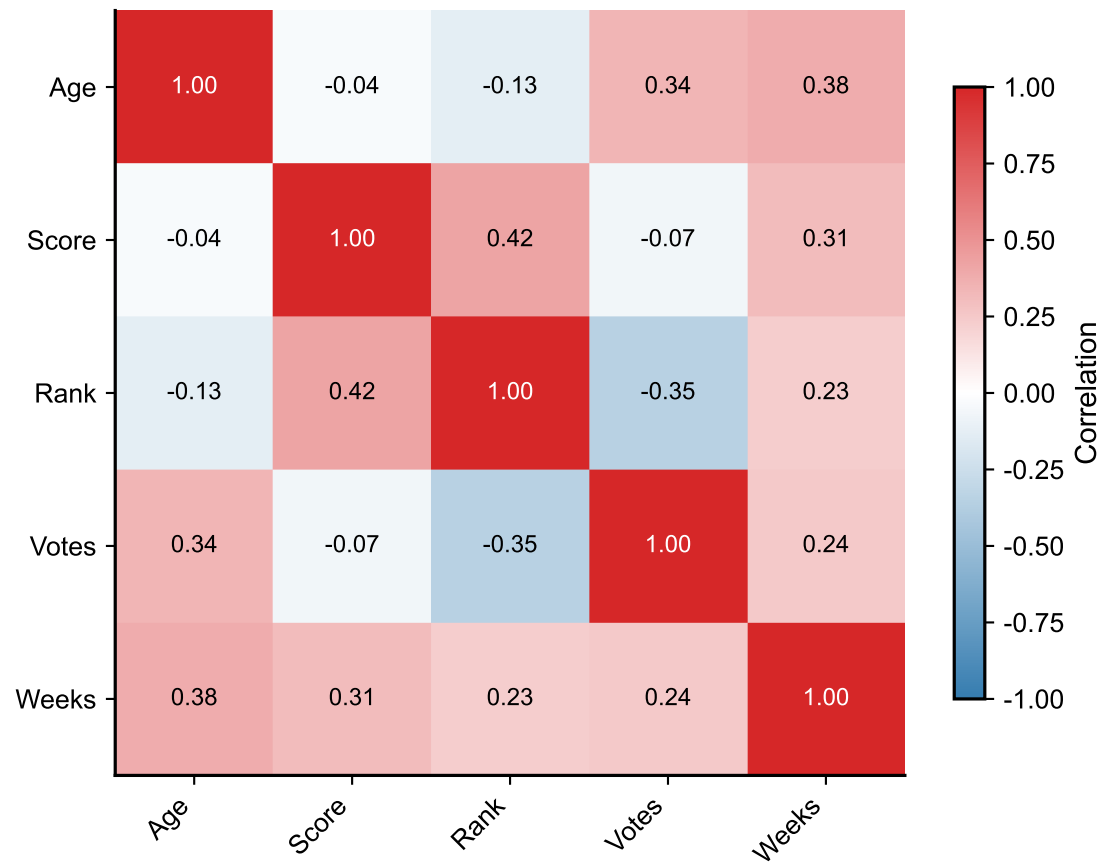
Correlation Matrix
