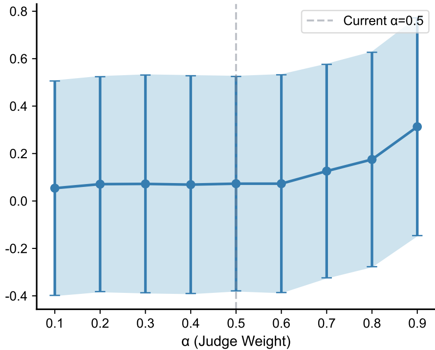
Rank Consistency with Judges
