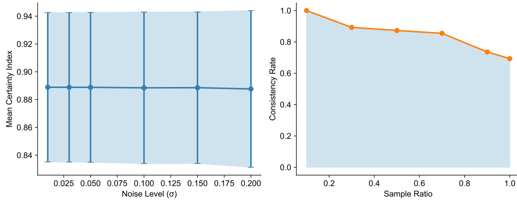
Figure 14: Sensitivity to noise level and sampling ratio.
