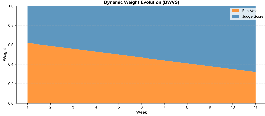
Figure 11: Dynamic weight evolution across competition weeks.
