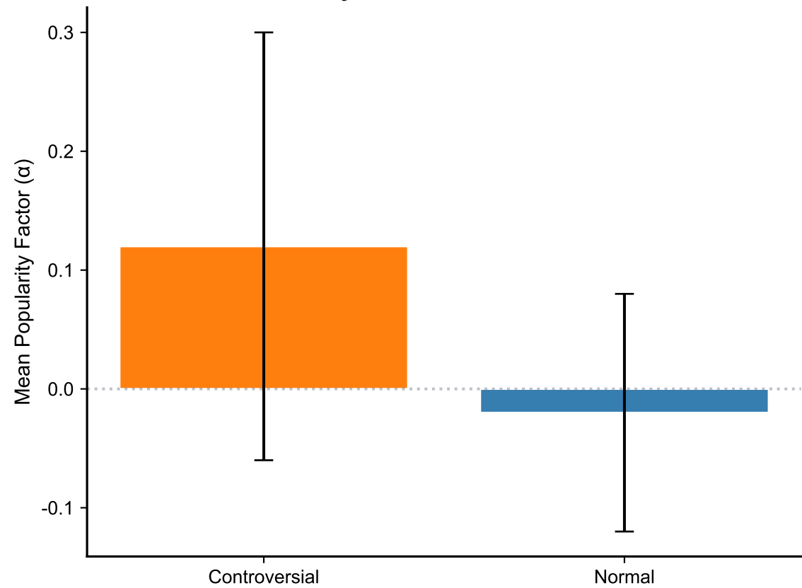
\alpha by Controversial Status
