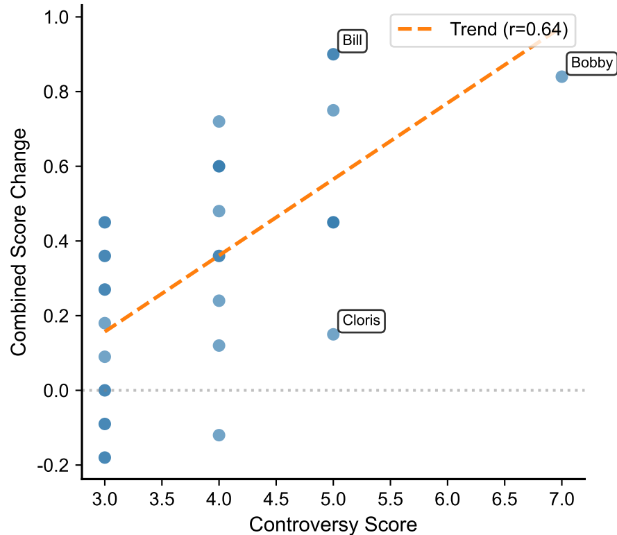
Controversy vs. DWVS Impact
