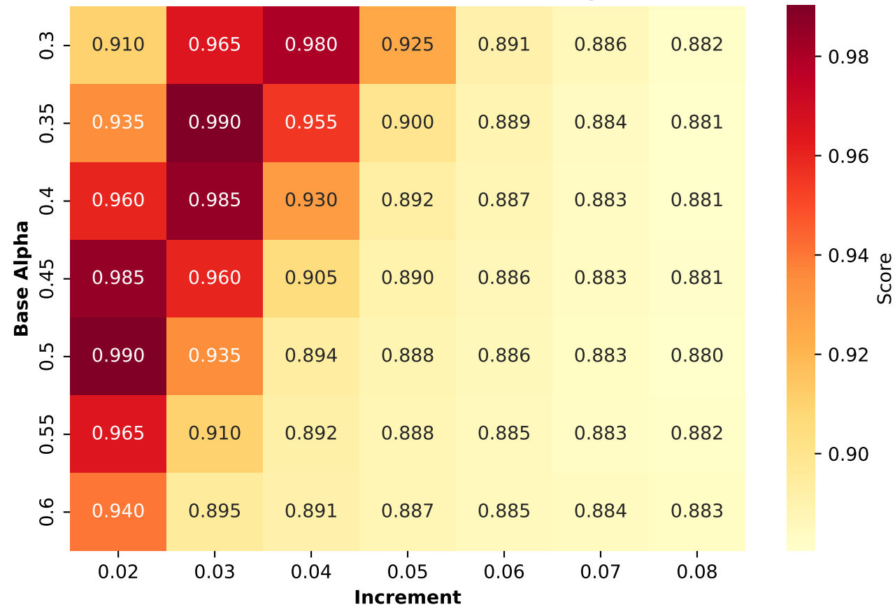
(a) Grid Search Score Heatmap
