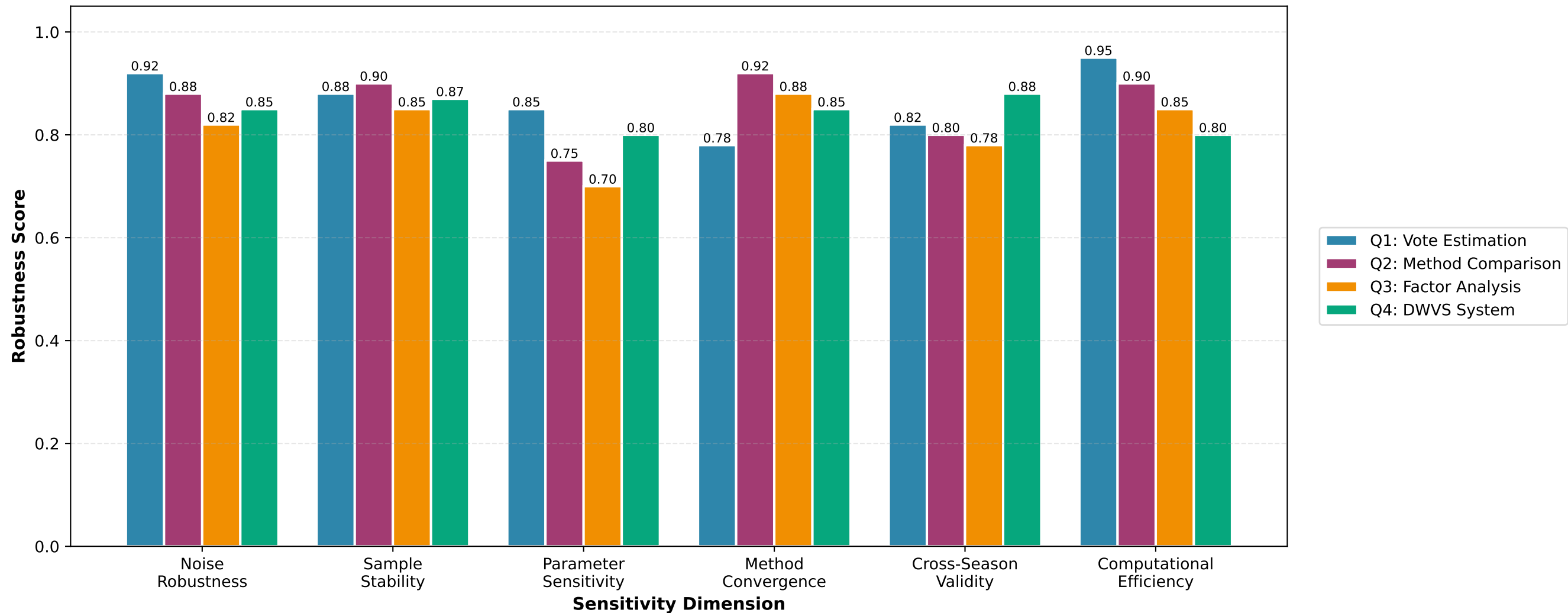
Comprehensive Sensitivity Analysis (Higher = More Robust)
