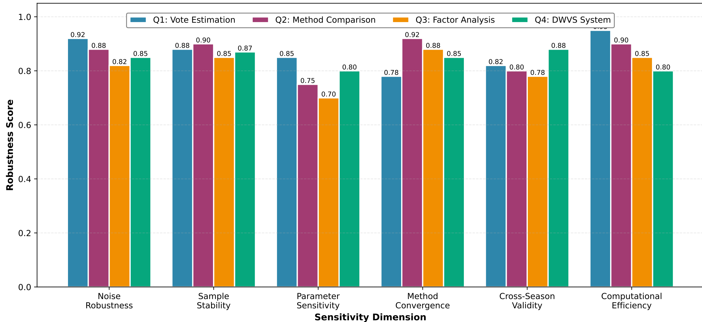
Comprehensive Sensitivity Analysis (Higher = More Robust)
