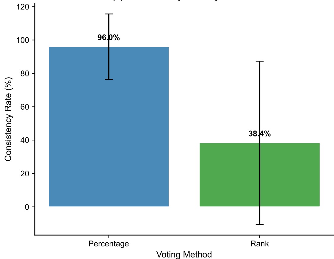
(b) Consistency Rate by Method
