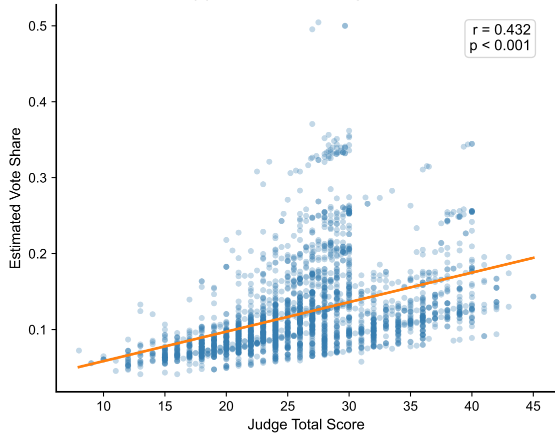
(a) Vote Share vs Judge Score
