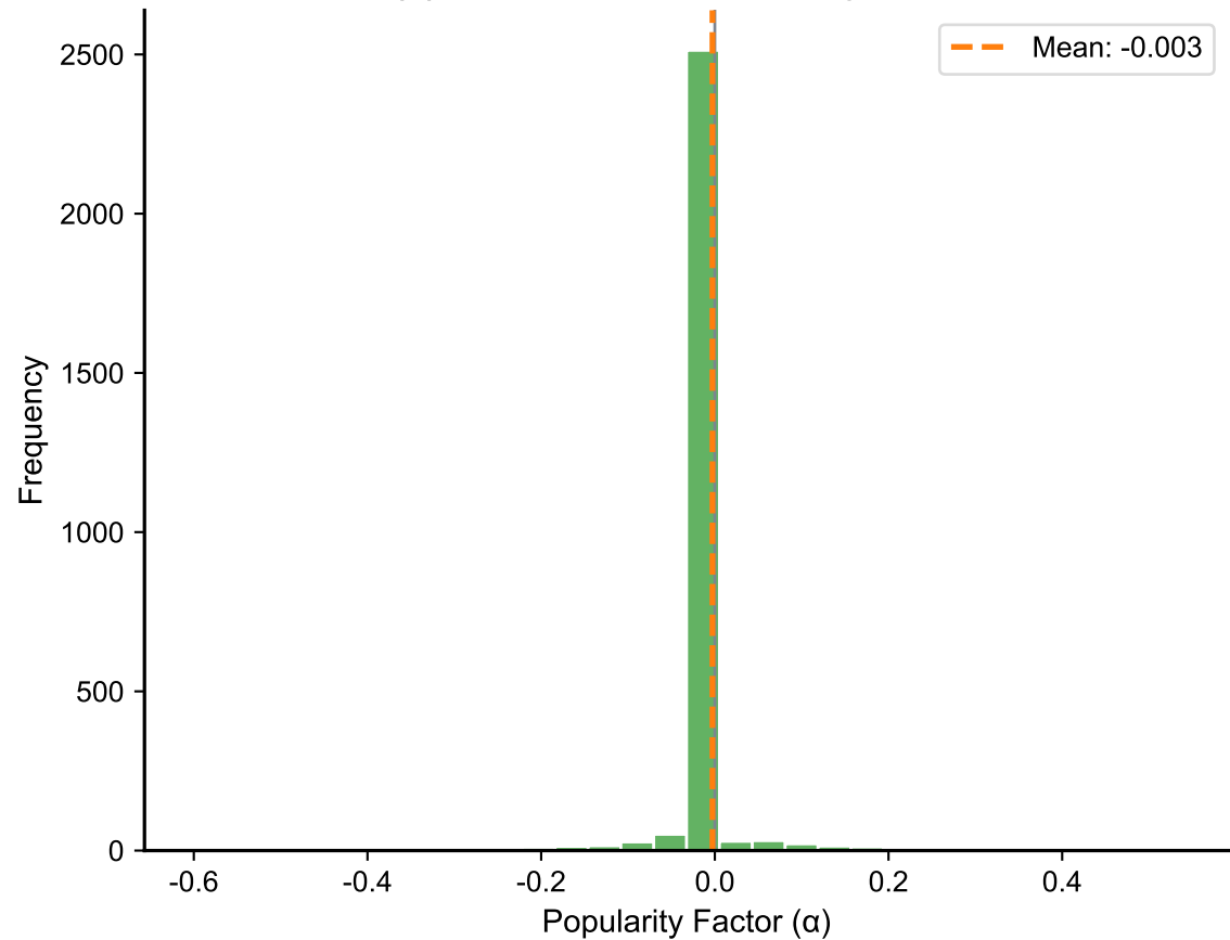
(b) Distribution of Popularity Factor
