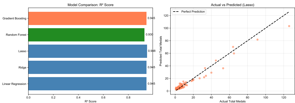
Figure 6: Model Performance Comparison
