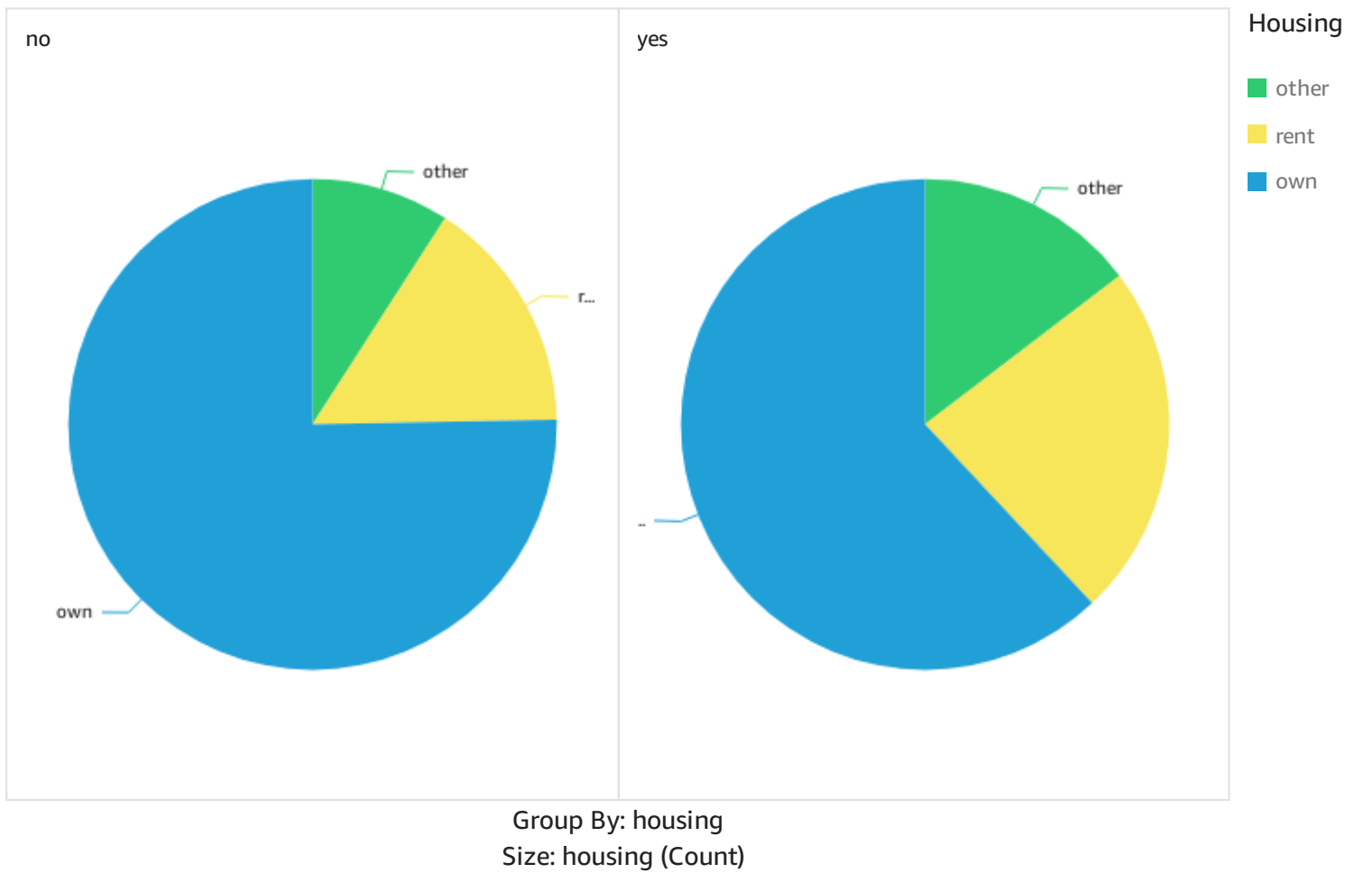
Housing distribution
