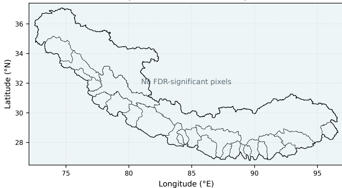
a Theil-Sen trend (native units decade -1 )
