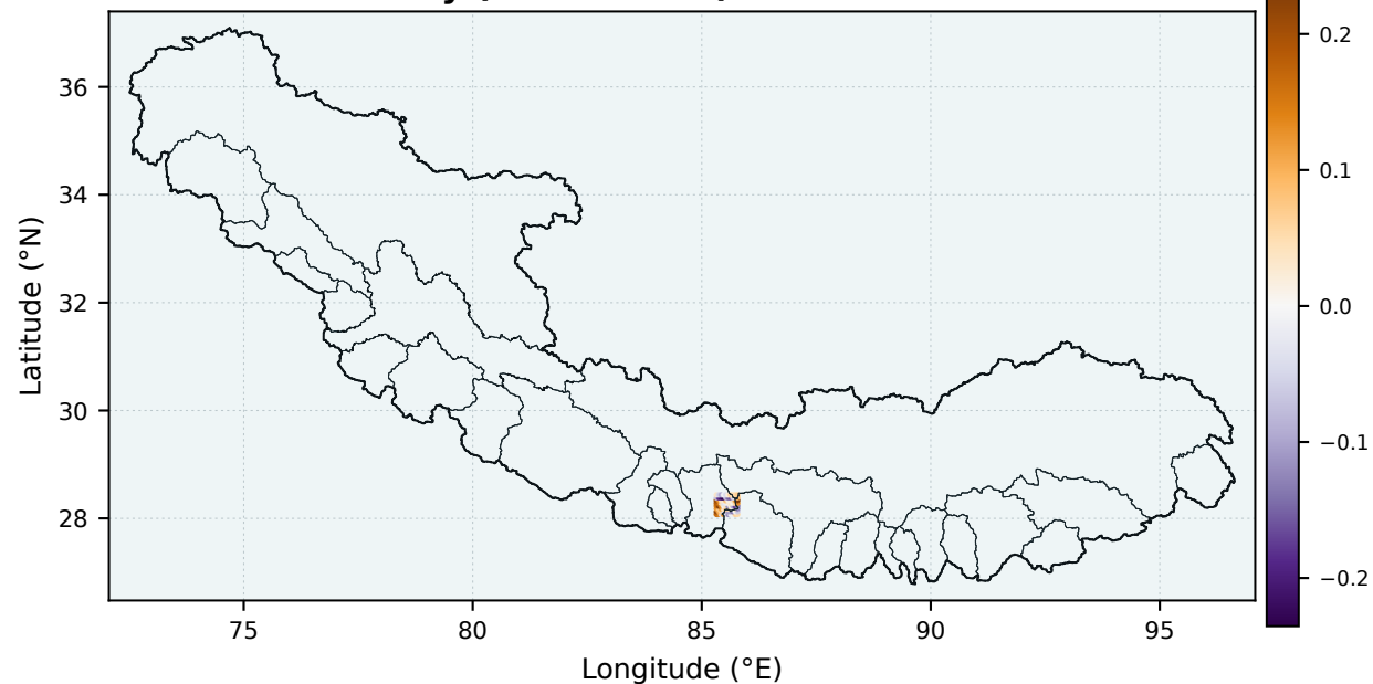
b Recent anomaly (baseline SD)
