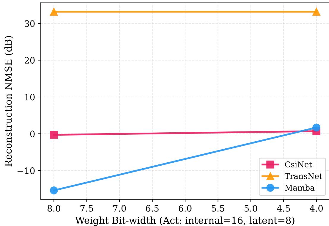
(b) Encoder Quantization Robustness
