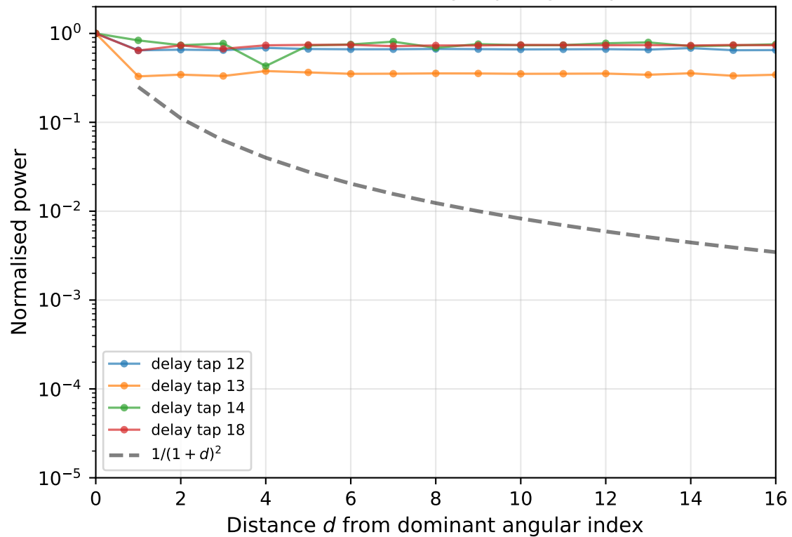
Outdoor: individual delay-tap angular profiles
