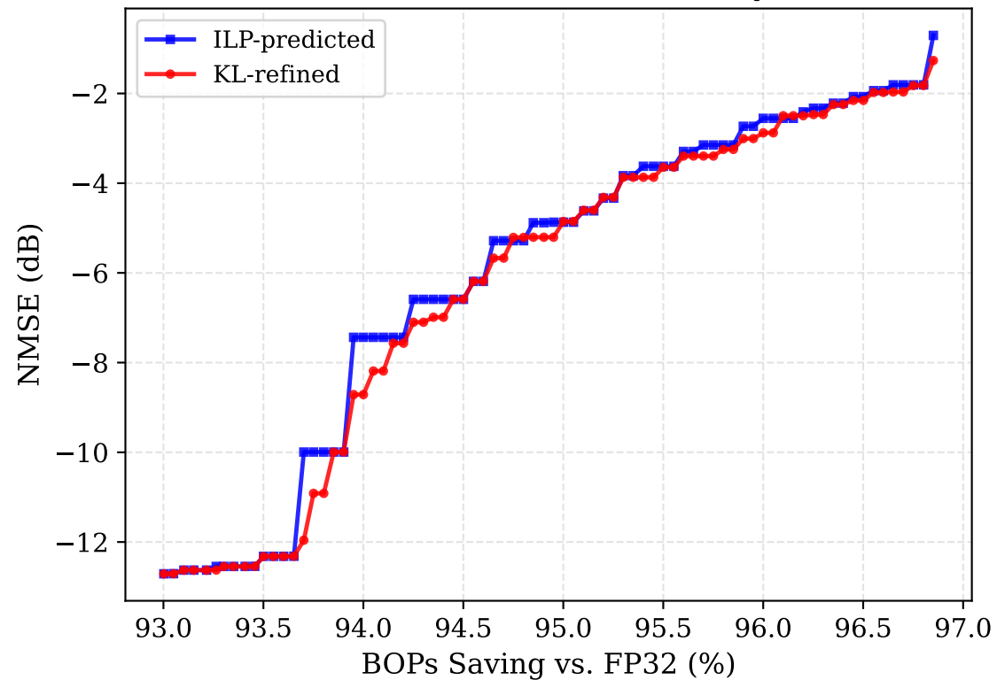
(a) ILP vs. KL-Refined Policy
