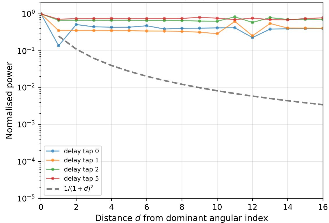
Indoor: individual delay-tap angular profiles
