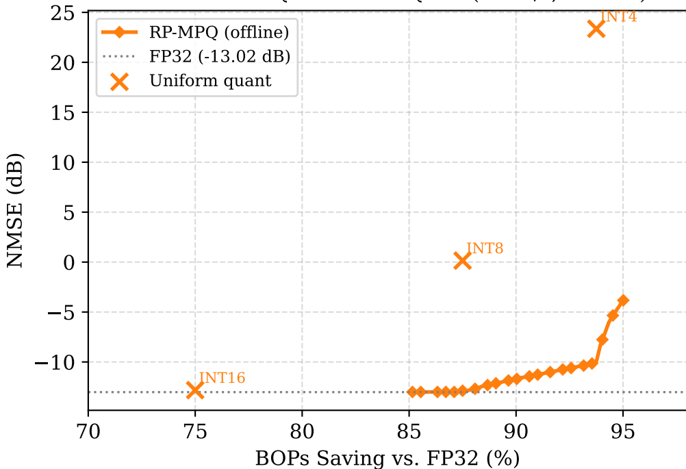
CLNet -- RP-MPQ vs. Uniform Quant (CR=1/4, Outdoor)
