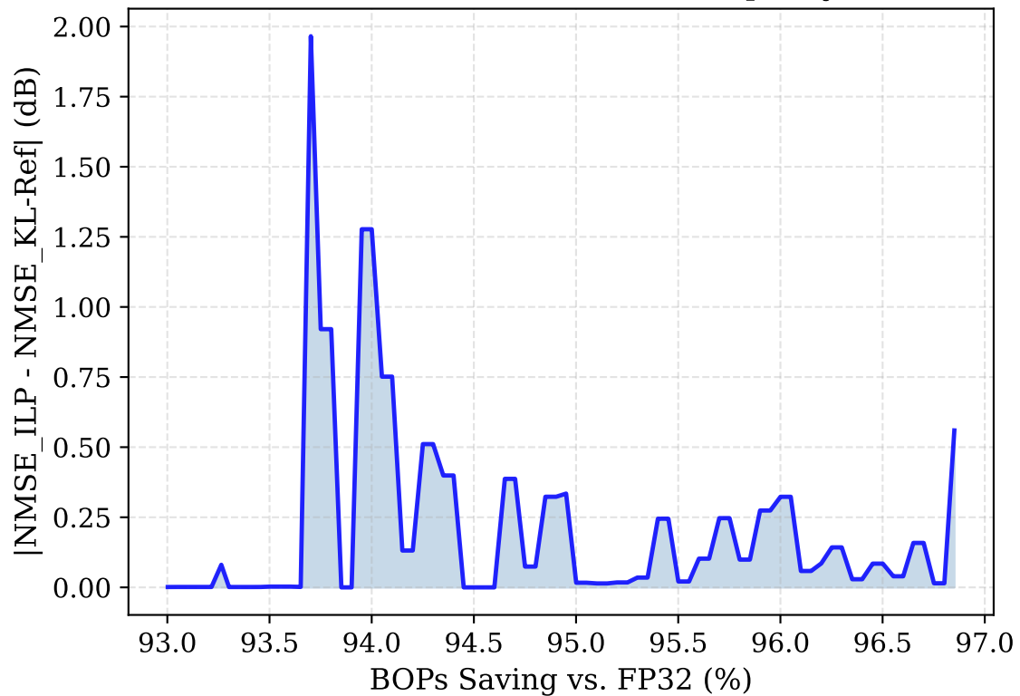
(b) ILP vs. KL-Refined Discrepancy
