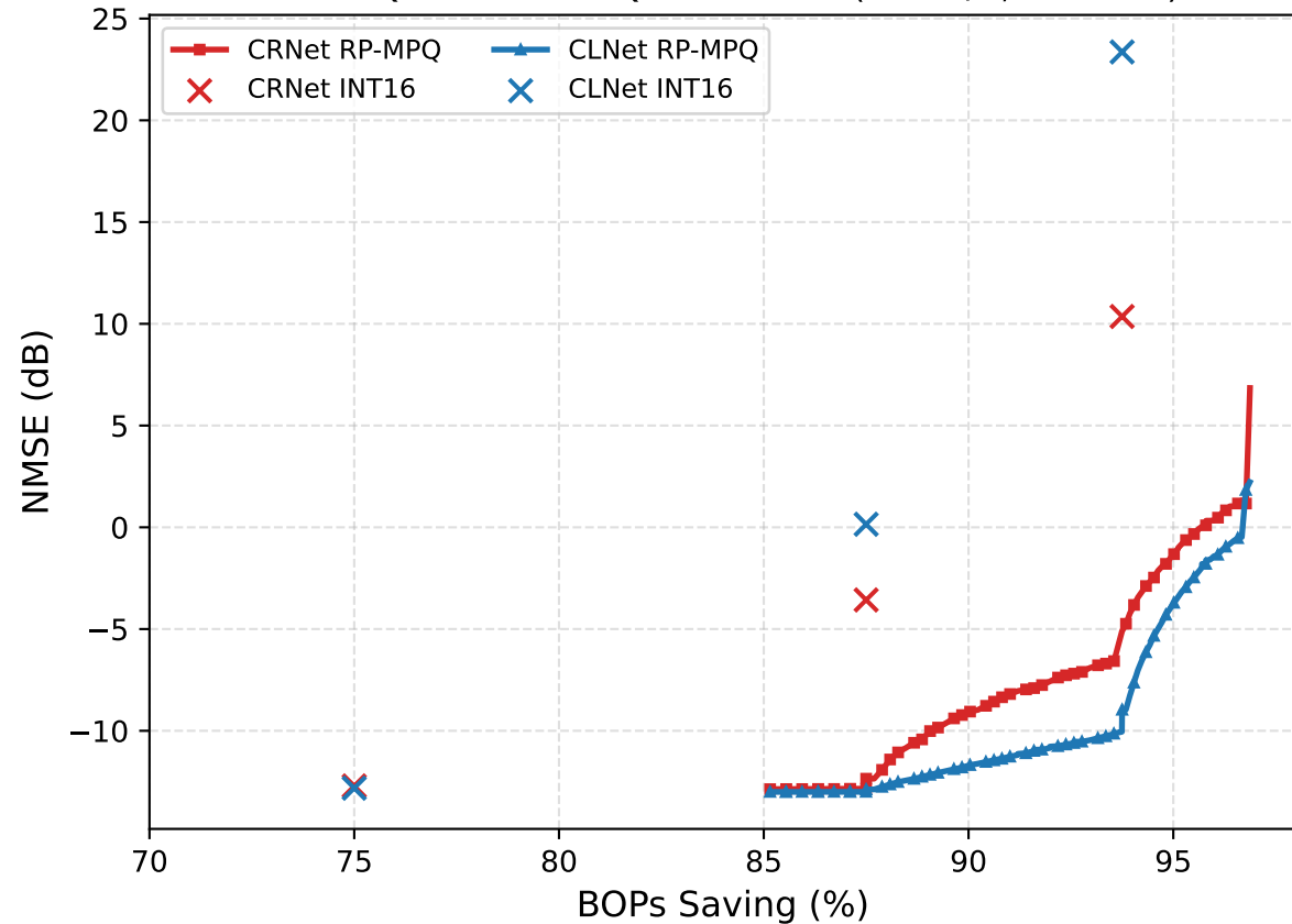
RP-MPQ vs Uniform Quantization (CR=1/4, Outdoor)
