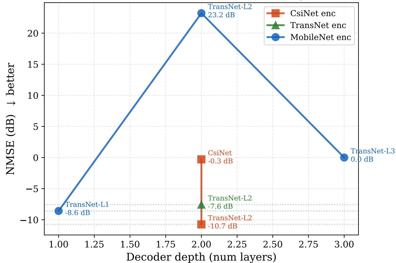
Encoder-Induced Information Floor (Eq. 10)
