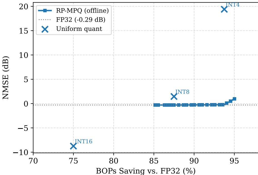
CsiNet -- RP-MPQ vs. Uniform Quant (CR=1/4, Outdoor)
