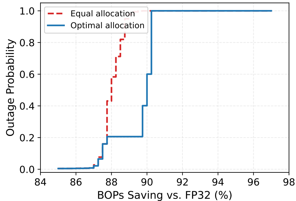
(a) SNR = 10 dB
