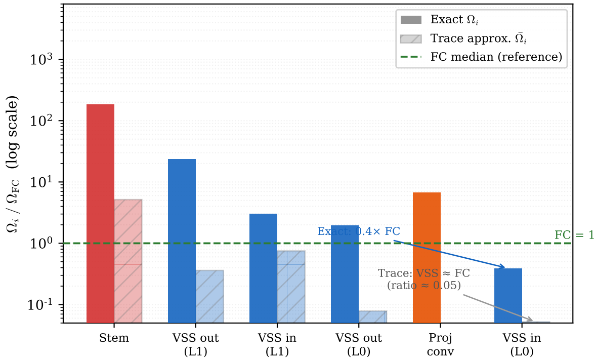
Inter-layer sensitivity ratio: exact \Omega_i vs trace approx. \bar{\Omega}_i (INT4)
