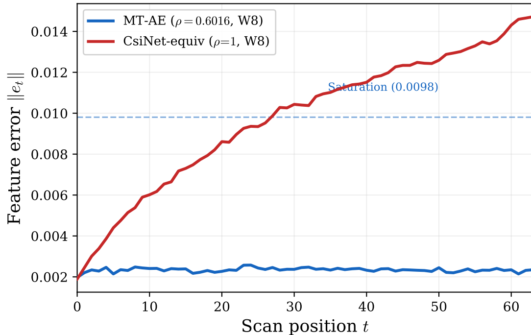
(b) W8: contractive vs non-contractive (synthetic) MT-AE ( \rho < 1 ) vs CsiNet ( \rho = 1 )
