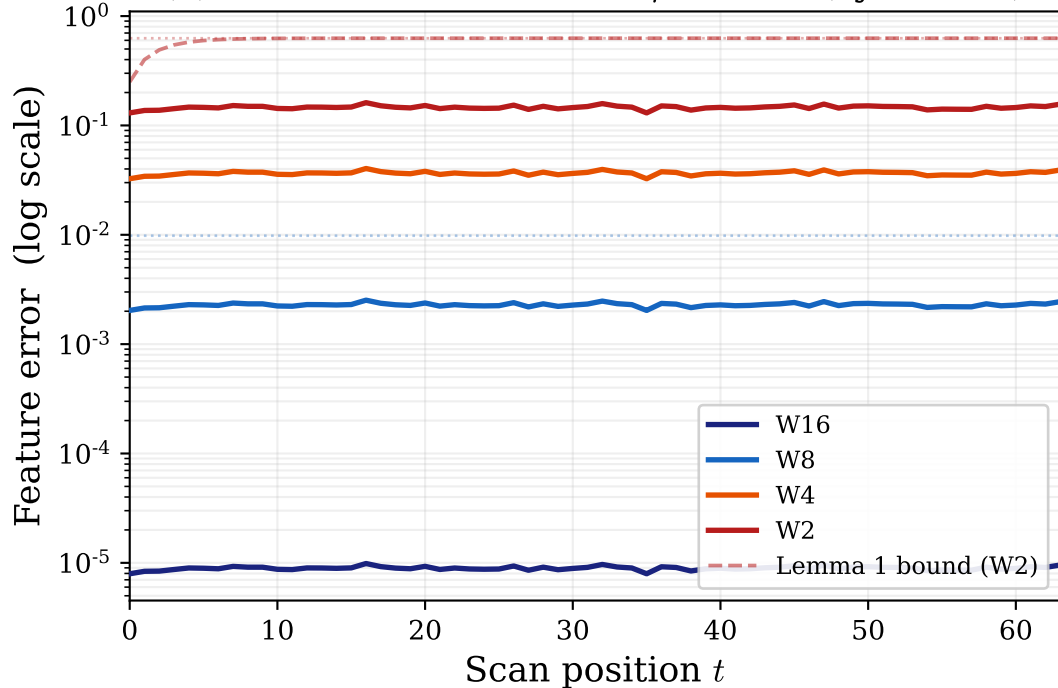
(a) SSM error saturation \rho = 0.6016 (synthetic)
