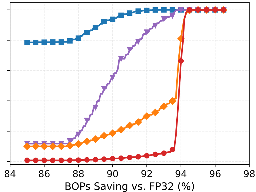
(b) \gamma = 0.98
