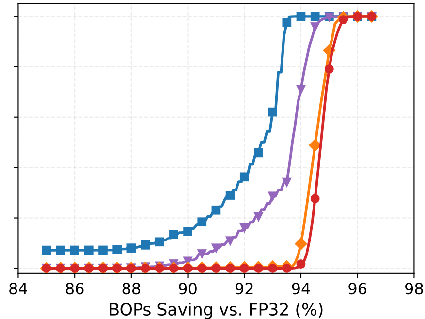
(c) \gamma = 0.95
