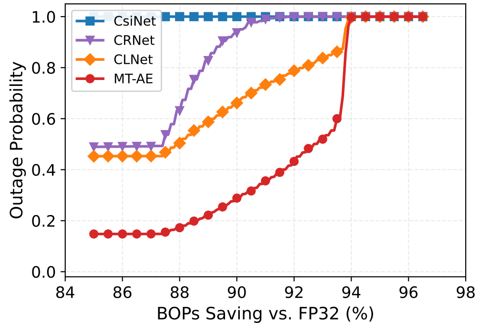
(a) \gamma = 0.99
