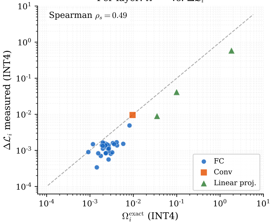
Per-layer: \Omega_i^{\text{exact}} vs. \Delta\mathcal{L}_i
