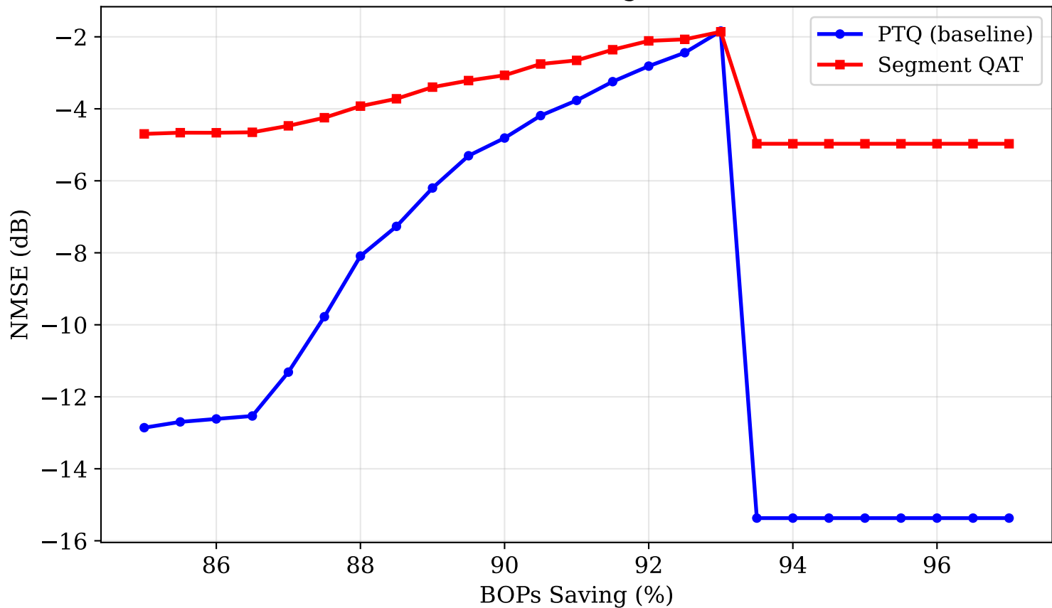
NMSE: PTQ vs Segment QAT
