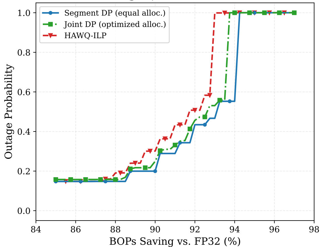
(b) Outage ( \gamma = 0.99 , SNR=20 dB)
