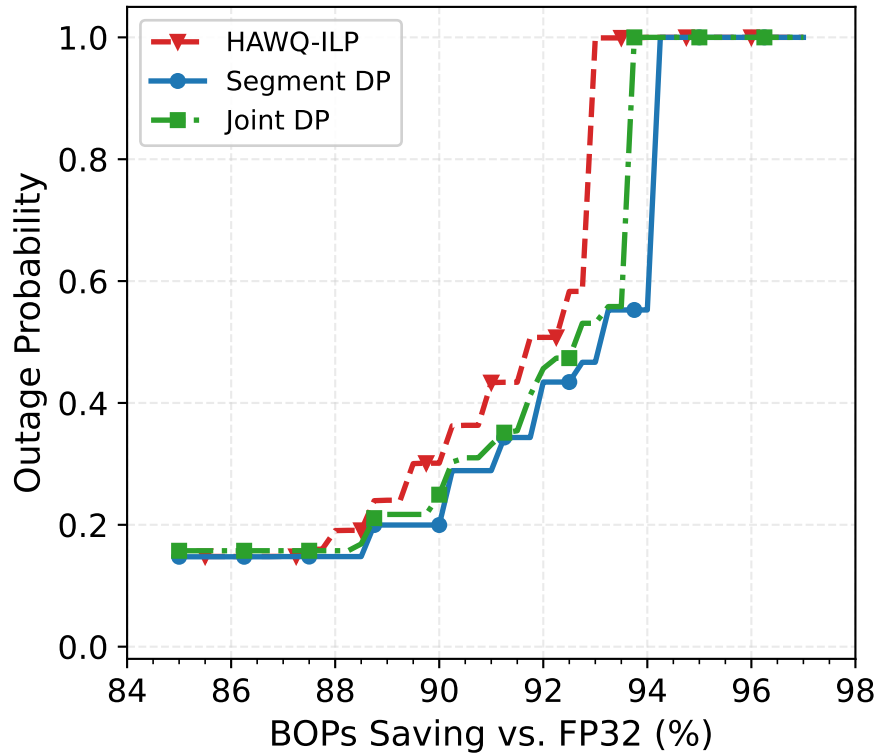
(b) Outage ( \gamma = 0.99 , SNR = 20 dB)
