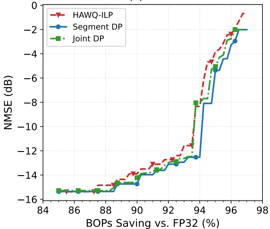
(a) NMSE
