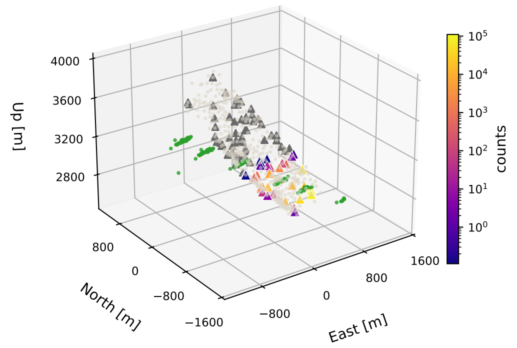
#282 (Emid/horiz) E=8.2e+05, \theta=86^\circ , \phi=115^\circ , 40/100
