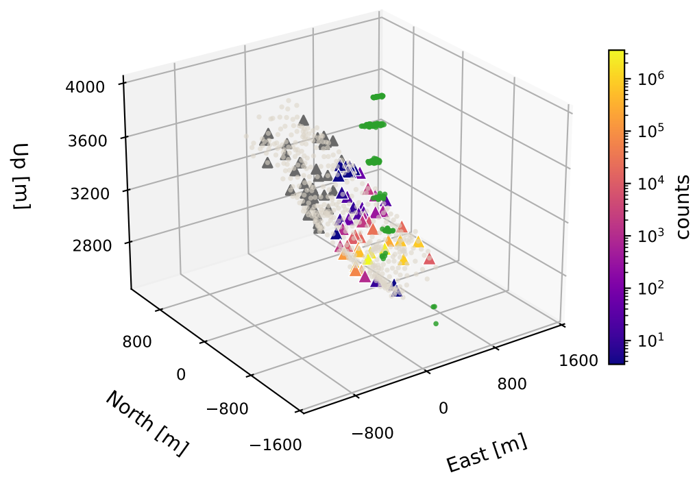
#275 (Ehigh/vert) E=5.4e+06, \theta=79^\circ , \phi=63^\circ , 60/100
