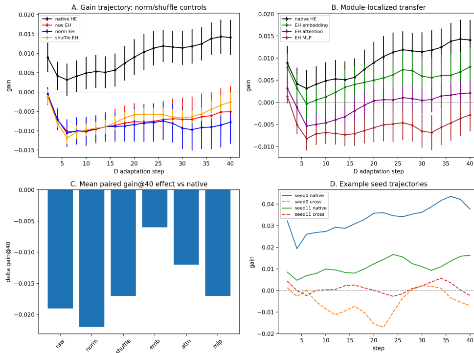
Figure 7: W_fast cross-injection and full future-adaptation trajectories. A: norm/shuffle controls. B: module-localized transfer. C: paired gain@40 effects. D: example trajectories.
