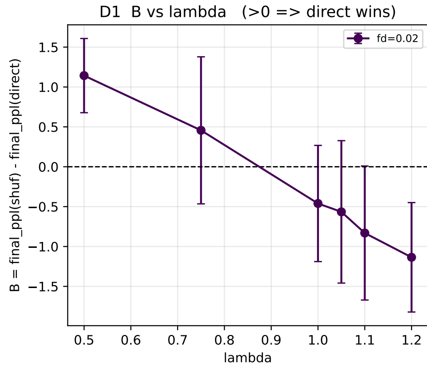
Figure D -- causal selective-writeback advantage
