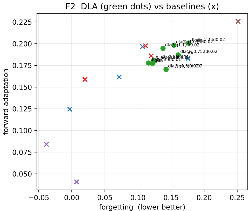
Figure F -- continual-learning position (DLA swept over (fast_decay, lambda), not a single tuned point)
