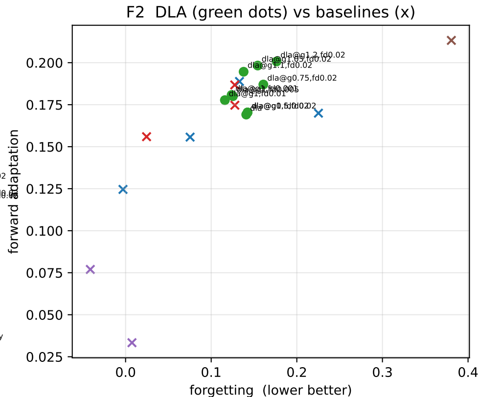
Figure F -- continual-learning position (DLA swept over (fast decay, lambda), not a single tuned point)
