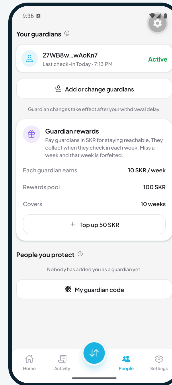
Rewards pool
