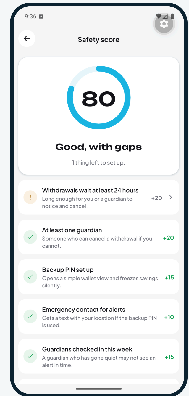
Safety score
