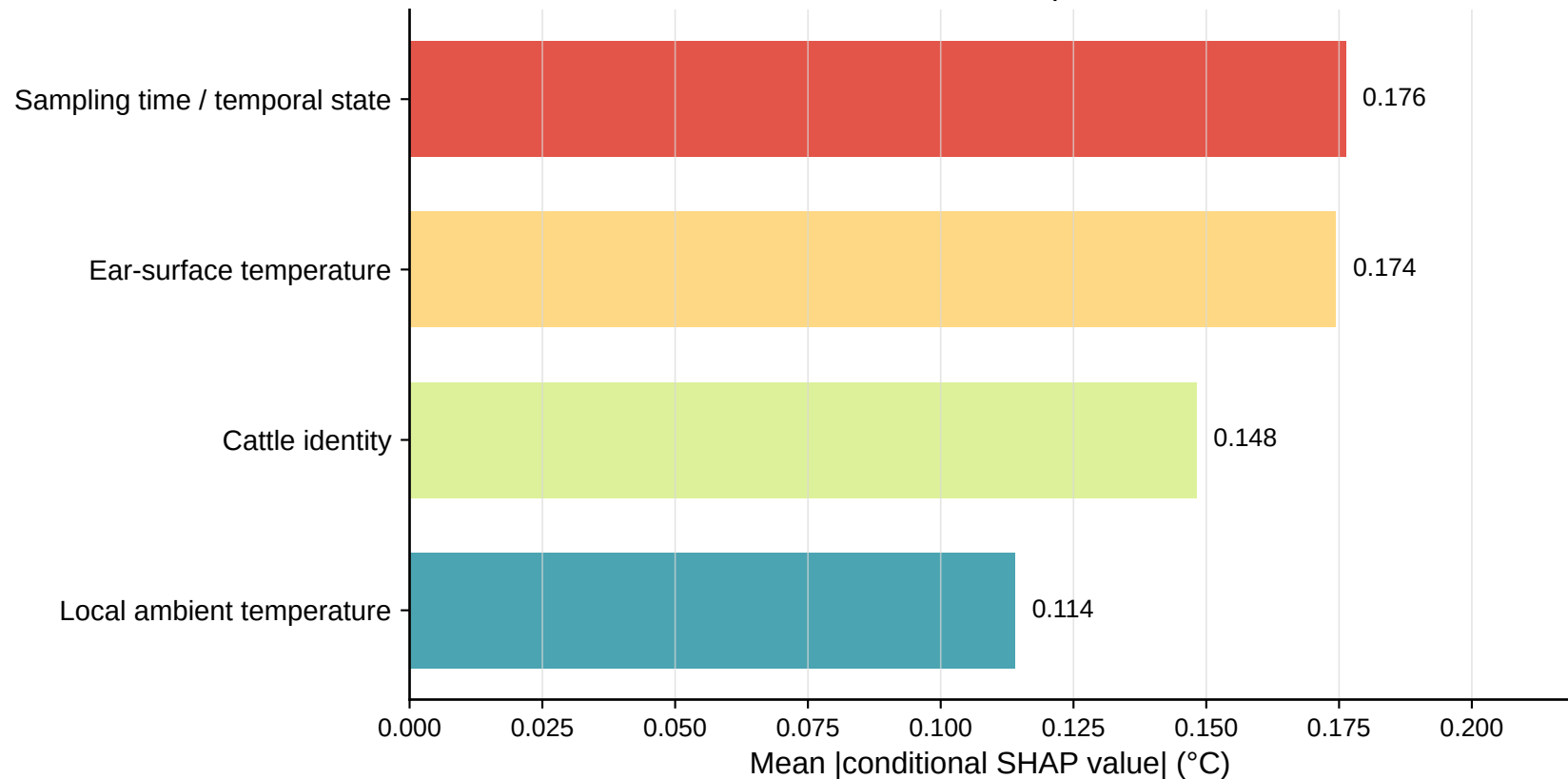
Global feature importance
