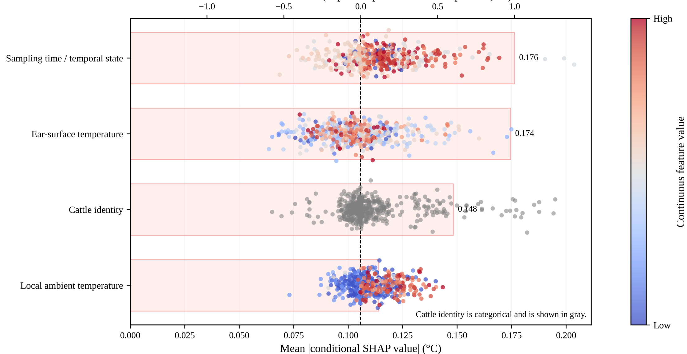
Conditional SHAP value (impact on predicted core temperature, °C)
