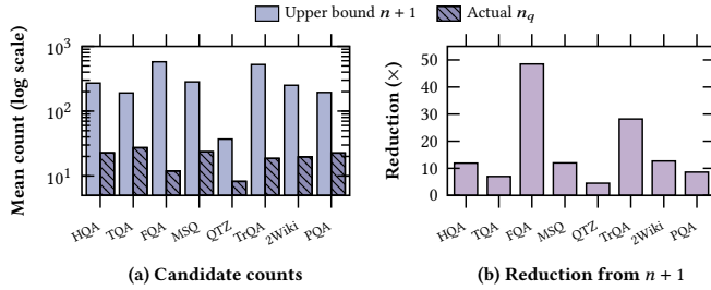
Figure 20: Candidate counts vs. the theoretical bound.
