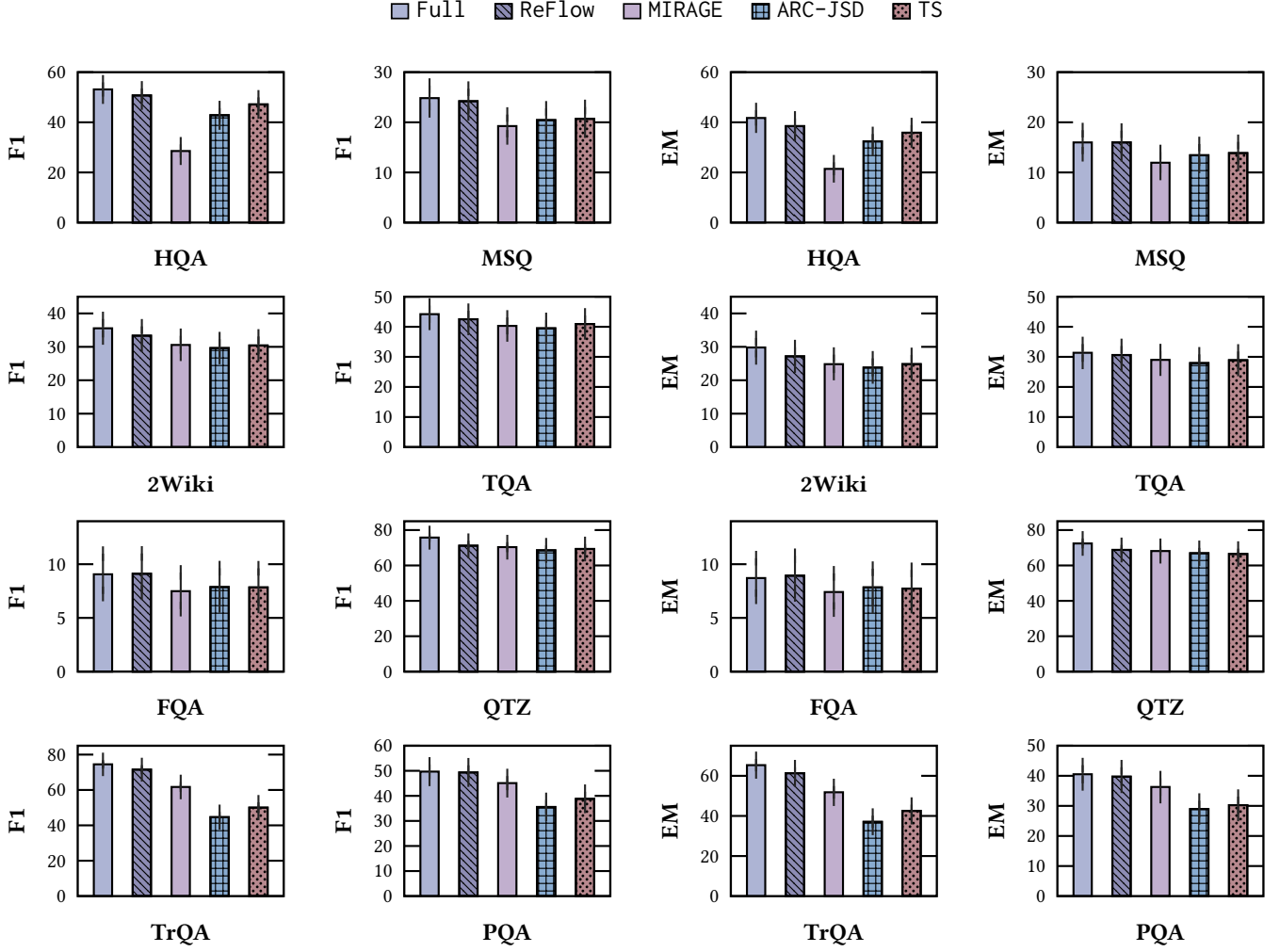
Figure 19: RAG provenance results on all eight datasets.
