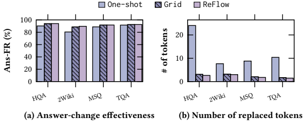
Figure 23: Comparison of token-selection strategies.
