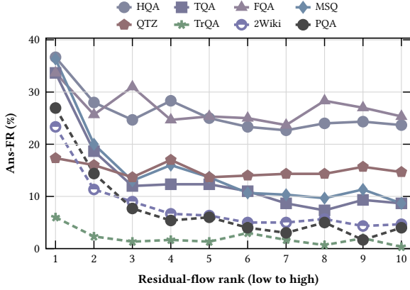
Figure 22: Residual-flow fidelity across eight datasets.
