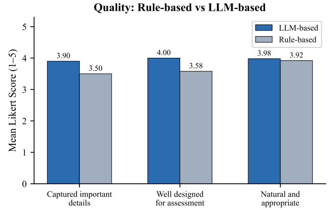
Fig. 5. Per-item Quality scores ( n = 40 ). The natural-and-appropriate item was nearly tied ( \Delta = +0.06 ), while other items showed larger differences.
