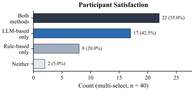
Fig. 6. Participant satisfaction endorsements (multi-select, n = 40 ). A majority endorsed both methods, with stronger endorsement for the LLM-based version.
