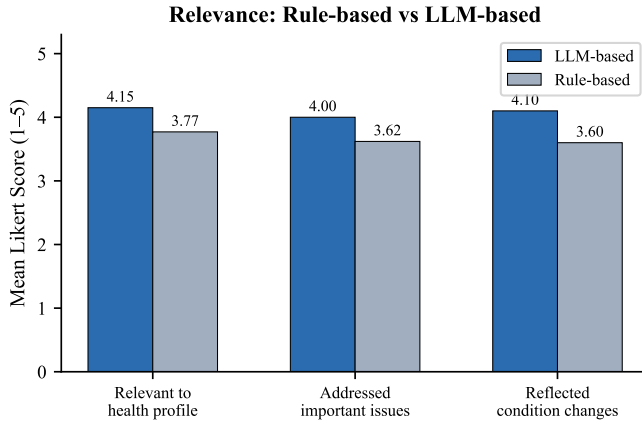
Fig. 4. Per-item Relevance scores ( n = 40 ). The LLM-based method showed the largest advantage on the change-tracking item ( \Delta = +0.50 ).
