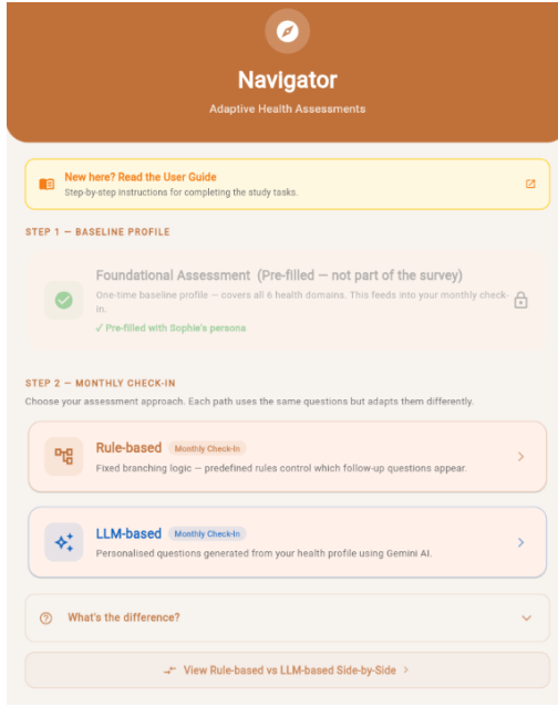
Fig. 1. Navigator prototype landing page. Step 1 shows the foundational assessment pre-filled with Sophie’s persona data; Step 2 presents the two monthly check-in methods.
